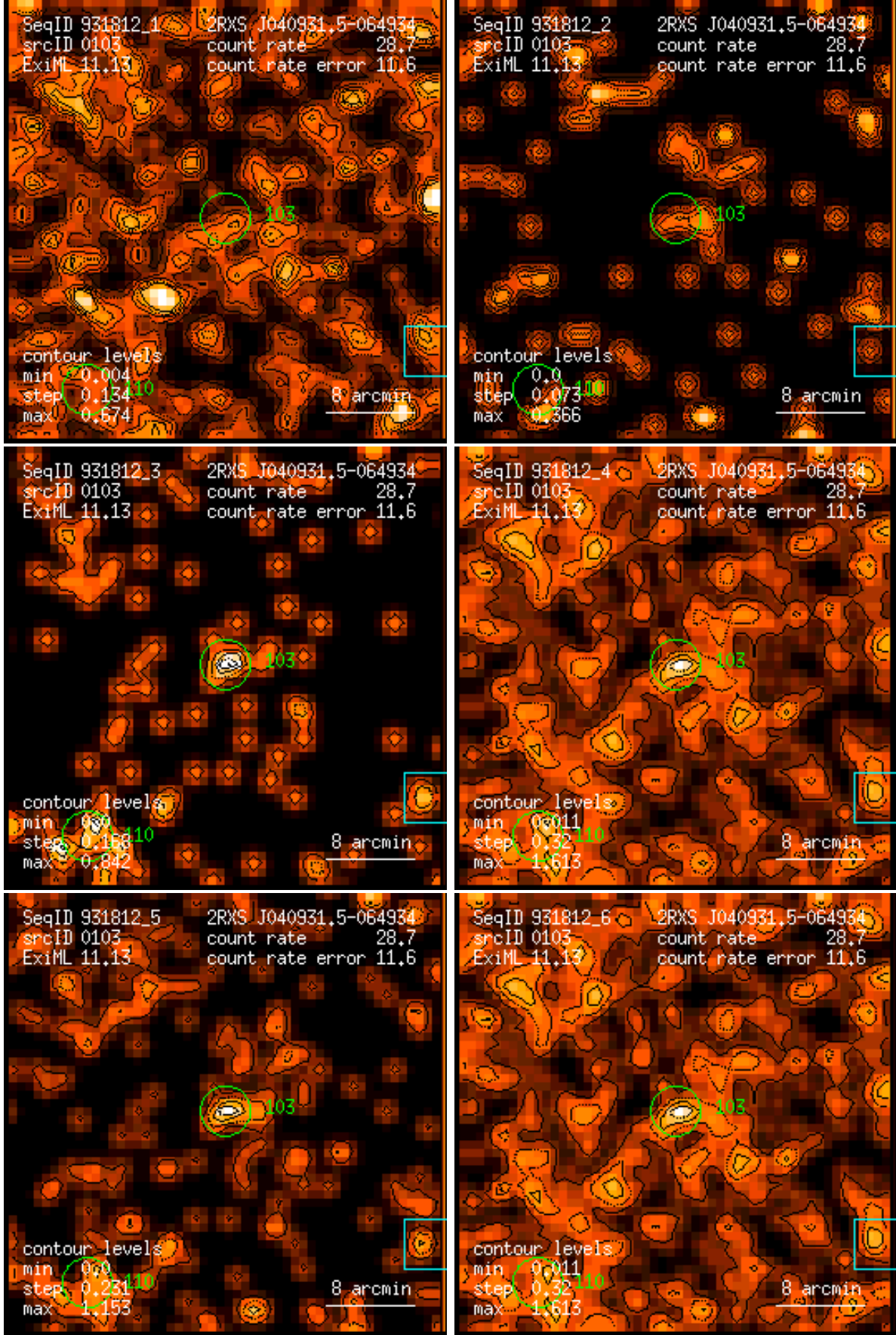
Figure 103: RASS 931812: detection 0103: band rate images, Gaussian filter: (1) PSPC channels 11 – 41, (2) 52 – 90, (3) 91 – 201, (4) 11 – 235, (5) 52 – 201, (6) 11 – 201. Broad band rates in counts/ks. Band rate contour levels in counts/ks/arcmin 2 .
