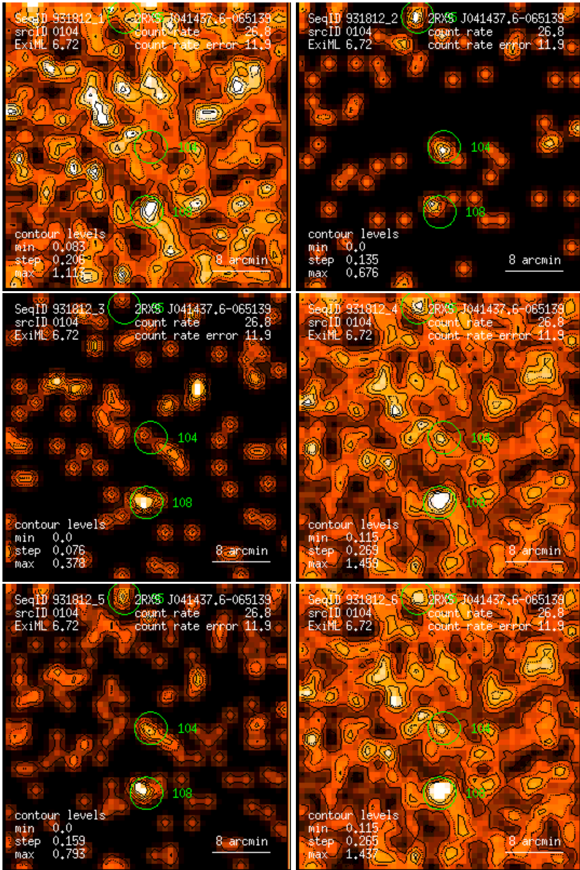
Figure 104: RASS 931812: detection 0104: band rate images, Gaussian filter: (1) PSPC channels 11 – 41, (2) 52 – 90, (3) 91 – 201, (4) 11 – 235, (5) 52 – 201, (6) 11 – 201. Broad band rates in counts/ks. Band rate contour levels in counts/ks/arcmin 2 .
