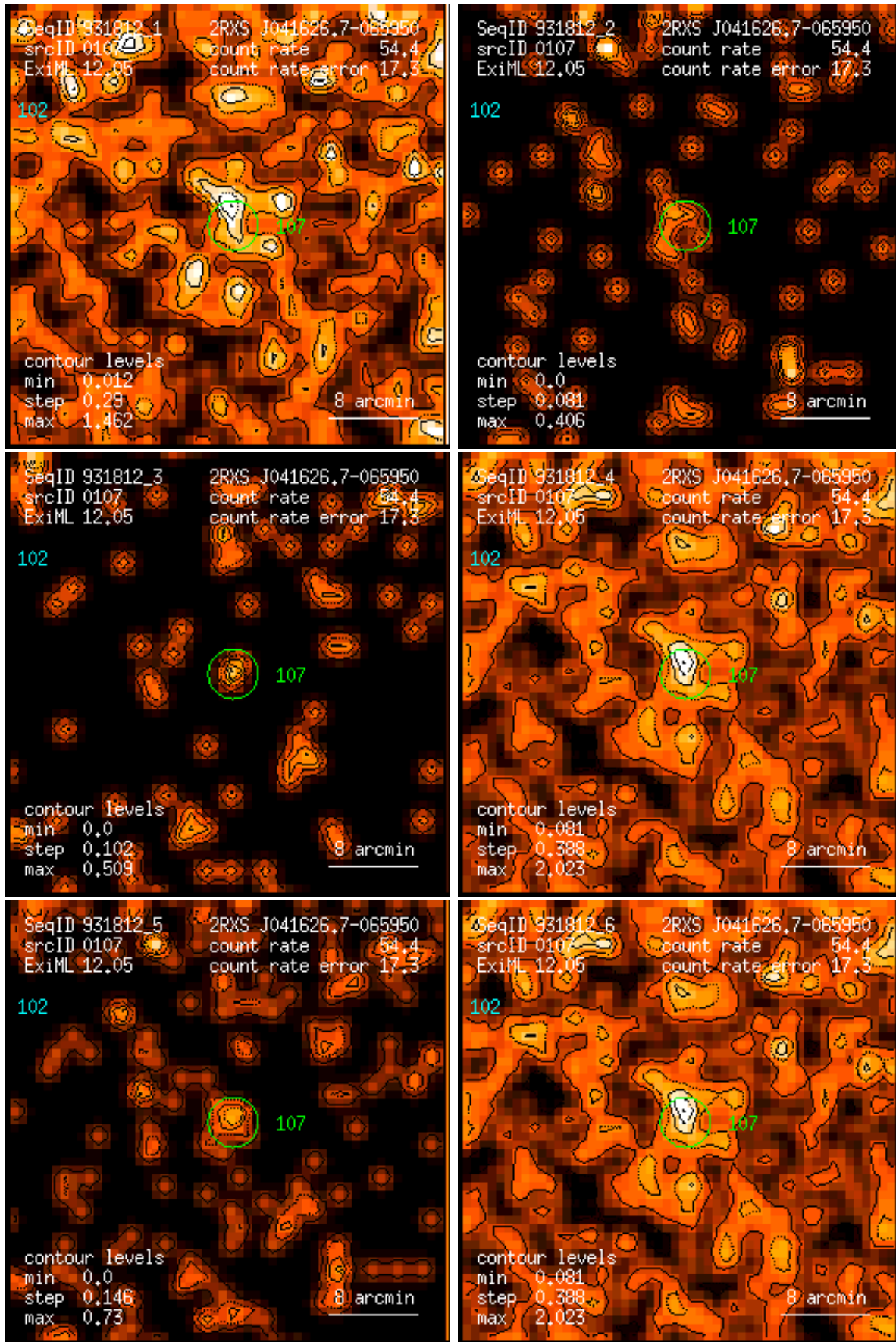
Figure 107: RASS 931812: detection 0107: band rate images, Gaussian filter: (1) PSPC channels 11 – 41, (2) 52 – 90, (3) 91 – 201, (4) 11 – 235, (5) 52 – 201, (6) 11 – 201. Broad band rates in counts/ks. Band rate contour levels in counts/ks/arcmin 2 .
