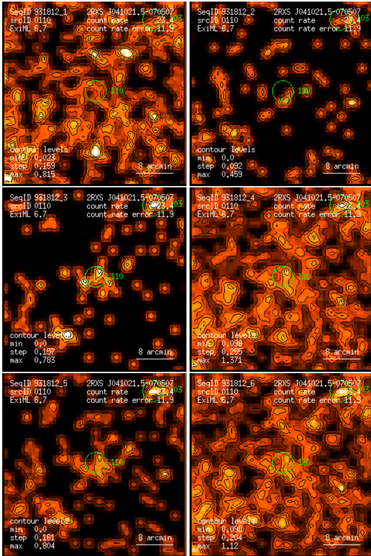
Figure 110: RASS 931812: detection 0110: band rate images, Gaussian filter: (1) PSPC channels 11 – 41, (2) 52 – 90, (3) 91 – 201, (4) 11 – 235, (5) 52 – 201, (6) 11 – 201. Broad band rates in counts/ks. Band rate contour levels in counts/ks/arcmin 2 .
