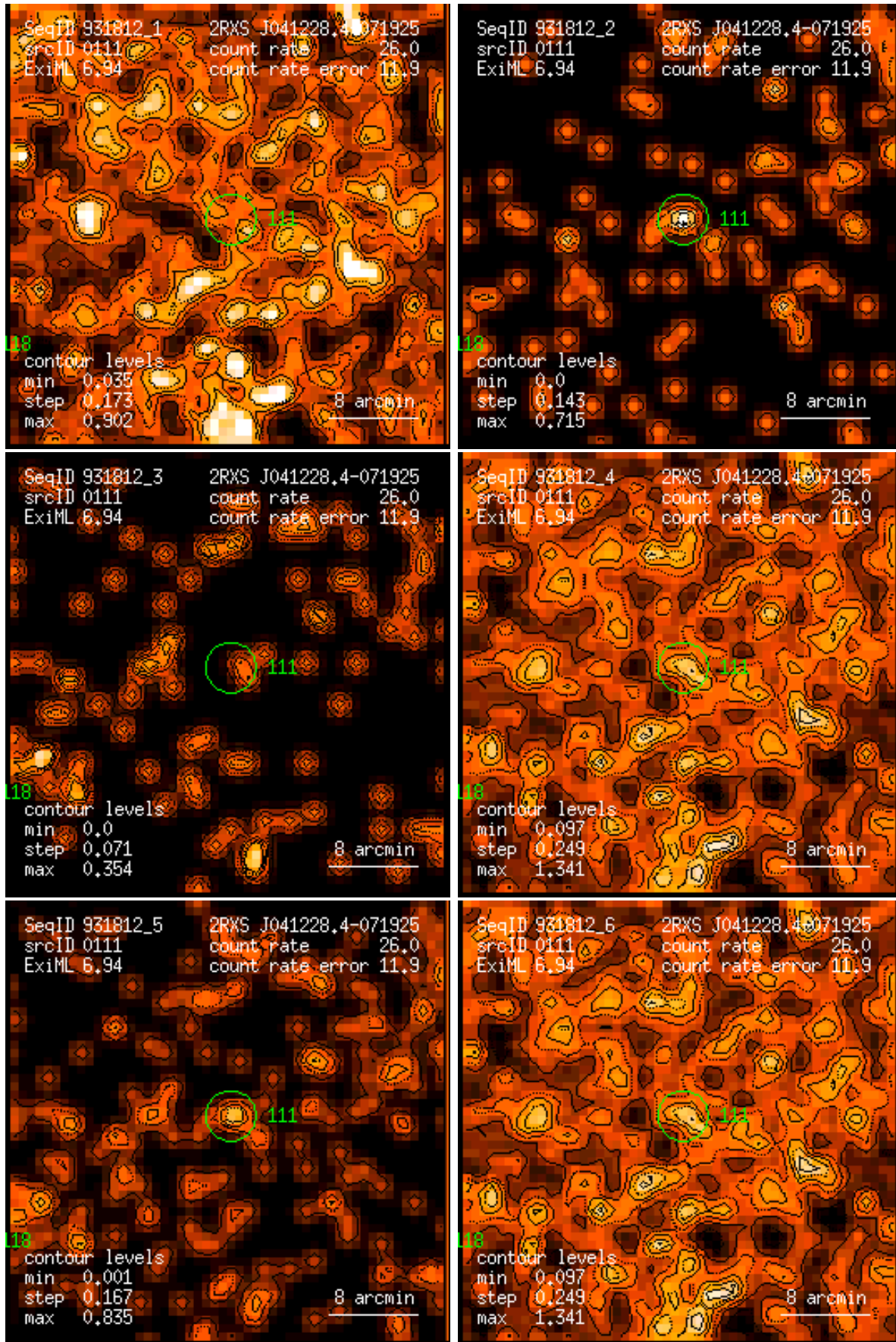
Figure 111: RASS 931812: detection 0111: band rate images, Gaussian filter: (1) PSPC channels 11 – 41, (2) 52 – 90, (3) 91 – 201, (4) 11 – 235, (5) 52 – 201, (6) 11 – 201. Broad band rates in counts/ks. Band rate contour levels in counts/ks/arcmin 2 .
