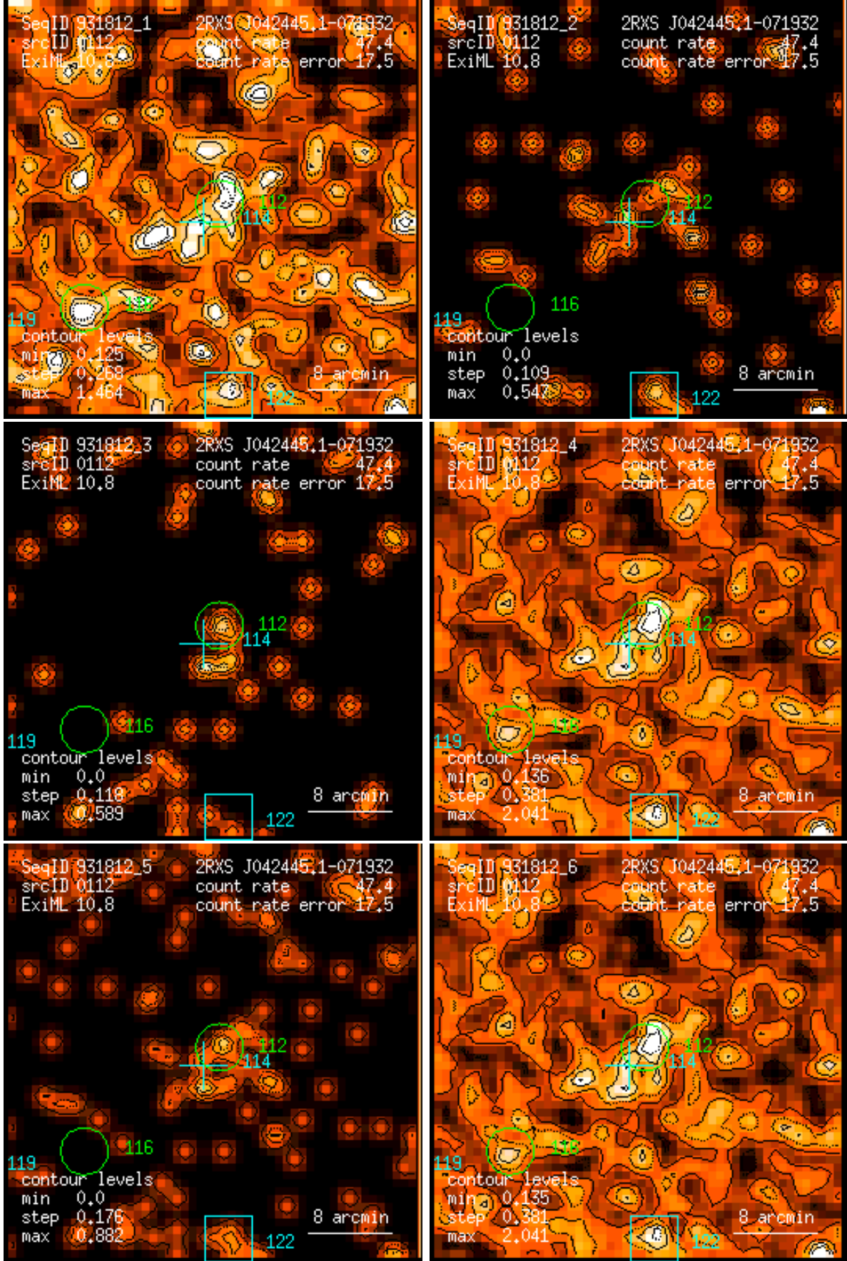
Figure 112: RASS 931812: detection 0112: band rate images, Gaussian filter: (1) PSPC channels 11 – 41, (2) 52 – 90, (3) 91 – 201, (4) 11 – 235, (5) 52 – 201, (6) 11 – 201. Broad band rates in counts/ks. Band rate contour levels in counts/ks/arcmin 2 .
