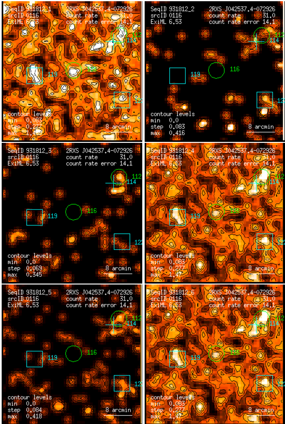
Figure 116: RASS 931812: detection 0116: band rate images, Gaussian filter: (1) PSPC channels 11 – 41, (2) 52 – 90, (3) 91 – 201, (4) 11 – 235, (5) 52 – 201, (6) 11 – 201. Broad band rates in counts/ks. Band rate contour levels in counts/ks/arcmin 2 .
