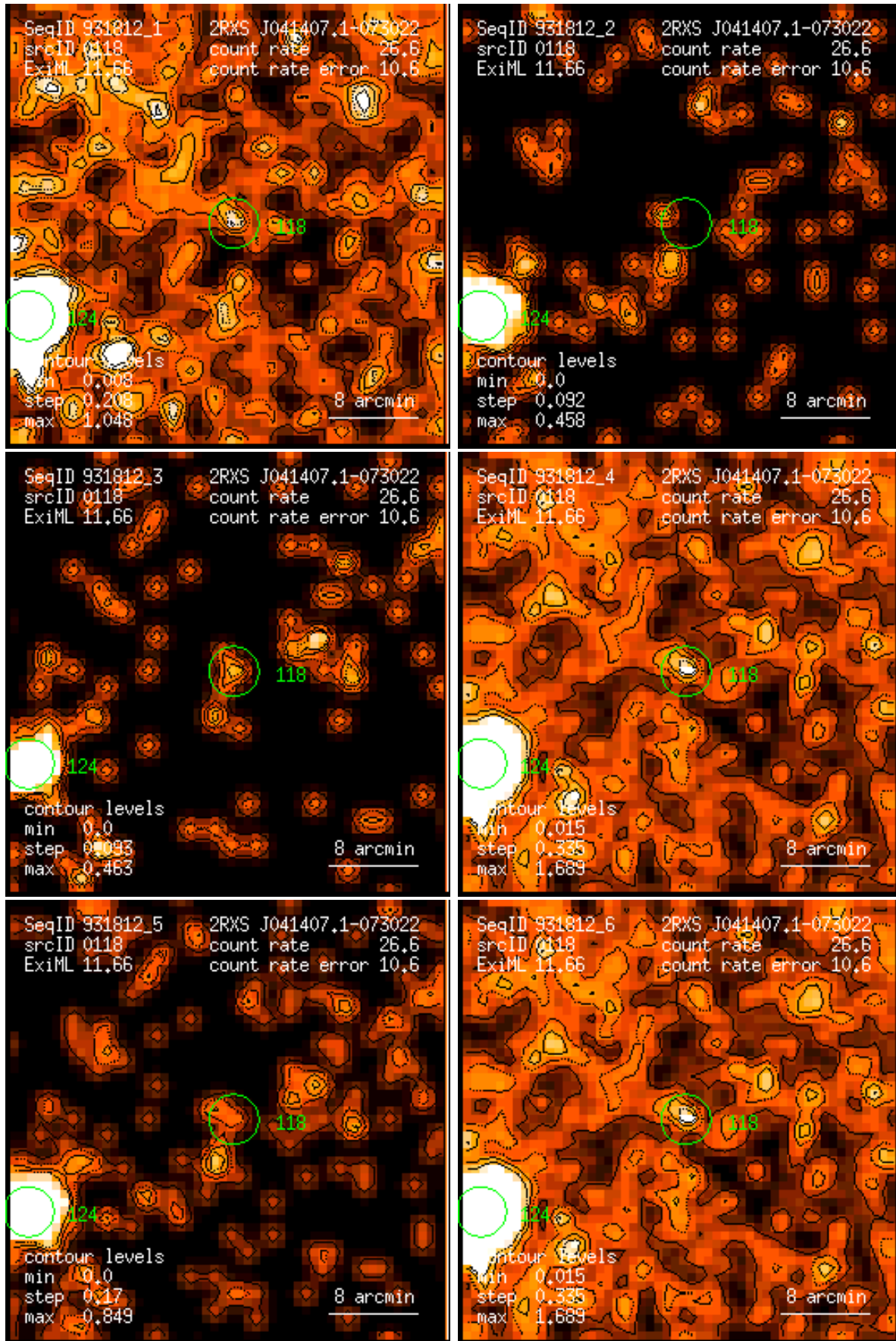
Figure 118: RASS 931812: detection 0118: band rate images, Gaussian filter: (1) PSPC channels 11 – 41, (2) 52 – 90, (3) 91 – 201, (4) 11 – 235, (5) 52 – 201, (6) 11 – 201. Broad band rates in counts/ks. Band rate contour levels in counts/ks/arcmin 2 .
