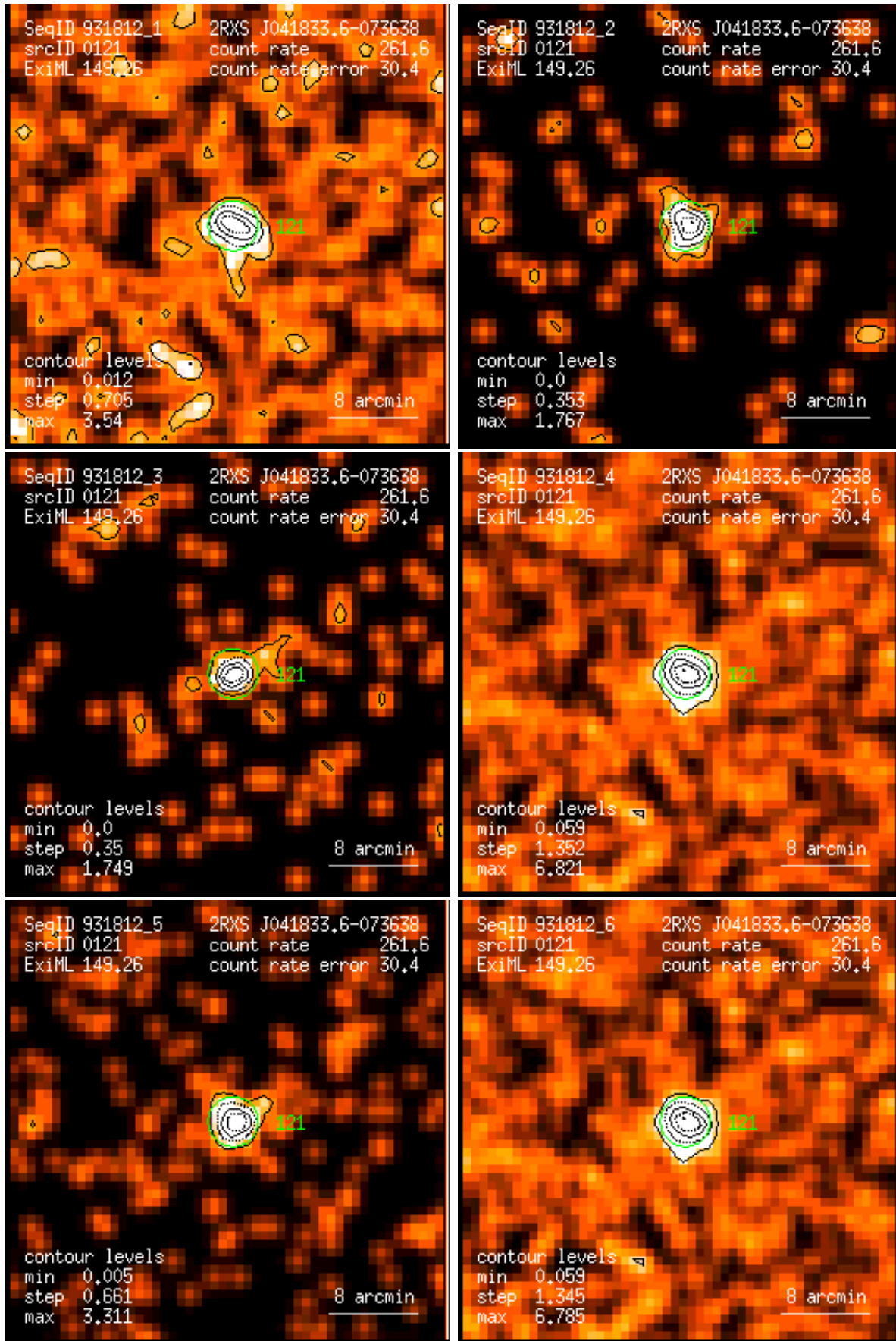
Figure 121: RASS 931812: detection 0121: band rate images, Gaussian filter: (1) PSPC channels 11 – 41, (2) 52 – 90, (3) 91 – 201, (4) 11 – 235, (5) 52 – 201, (6) 11 – 201. Broad band rates in counts/ks. Band rate contour levels in counts/ks/arcmin 2 .
