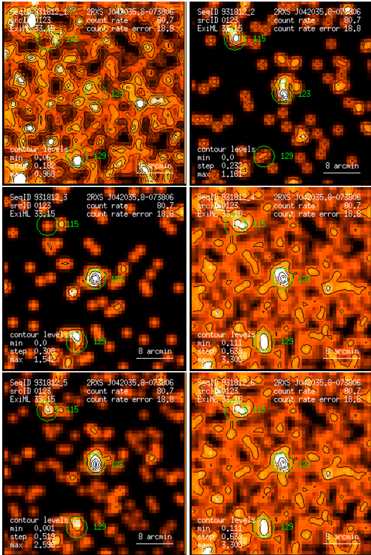
Figure 123: RASS 931812: detection 0123: band rate images, Gaussian filter: (1) PSPC channels 11 – 41, (2) 52 – 90, (3) 91 – 201, (4) 11 – 235, (5) 52 – 201, (6) 11 – 201. Broad band rates in counts/ks. Band rate contour levels in counts/ks/arcmin 2 .
