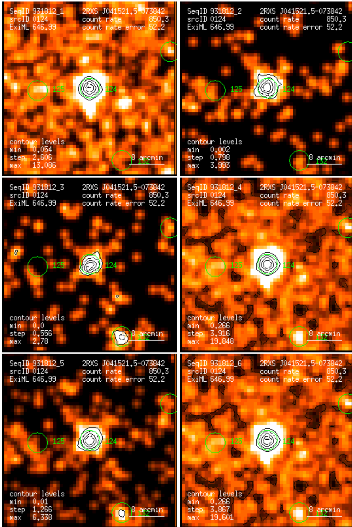
Figure 124: RASS 931812: detection 0124: band rate images, Gaussian filter: (1) PSPC channels 11 – 41, (2) 52 – 90, (3) 91 – 201, (4) 11 – 235, (5) 52 – 201, (6) 11 – 201. Broad band rates in counts/ks. Band rate contour levels in counts/ks/arcmin 2 .
