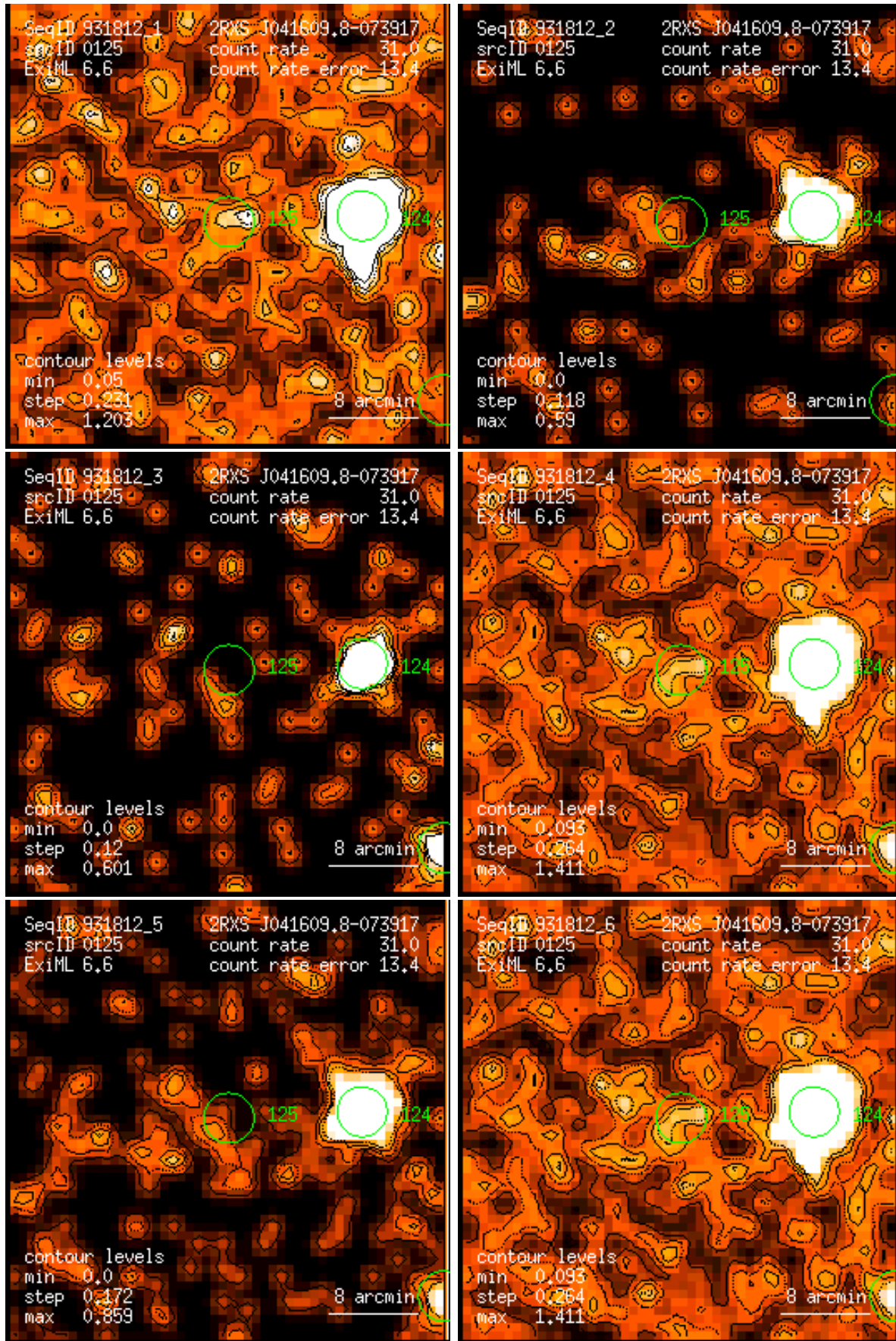
Figure 125: RASS 931812: detection 0125: band rate images, Gaussian filter: (1) PSPC channels 11 – 41, (2) 52 – 90, (3) 91 – 201, (4) 11 – 235, (5) 52 – 201, (6) 11 – 201. Broad band rates in counts/ks. Band rate contour levels in counts/ks/arcmin 2 .
