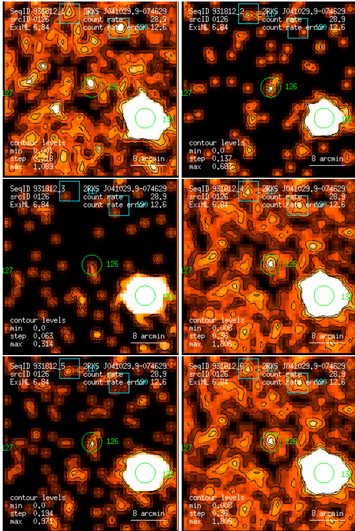
Figure 126: RASS 931812: detection 0126: band rate images, Gaussian filter: (1) PSPC channels 11 – 41, (2) 52 – 90, (3) 91 – 201, (4) 11 – 235, (5) 52 – 201, (6) 11 – 201. Broad band rates in counts/ks. Band rate contour levels in counts/ks/arcmin 2 .
