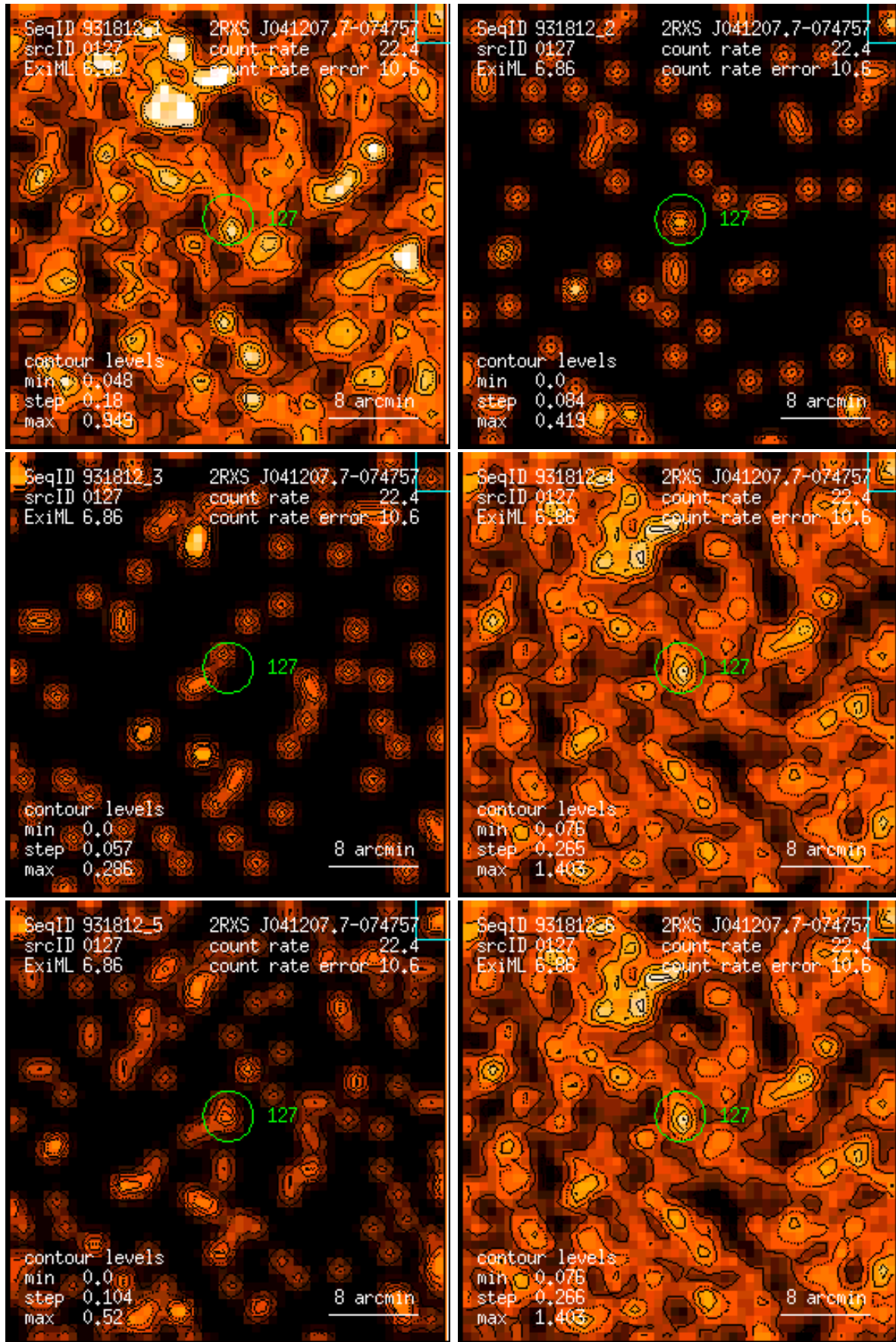
Figure 127: RASS 931812: detection 0127: band rate images, Gaussian filter: (1) PSPC channels 11 – 41, (2) 52 – 90, (3) 91 – 201, (4) 11 – 235, (5) 52 – 201, (6) 11 – 201. Broad band rates in counts/ks. Band rate contour levels in counts/ks/arcmin 2 .
