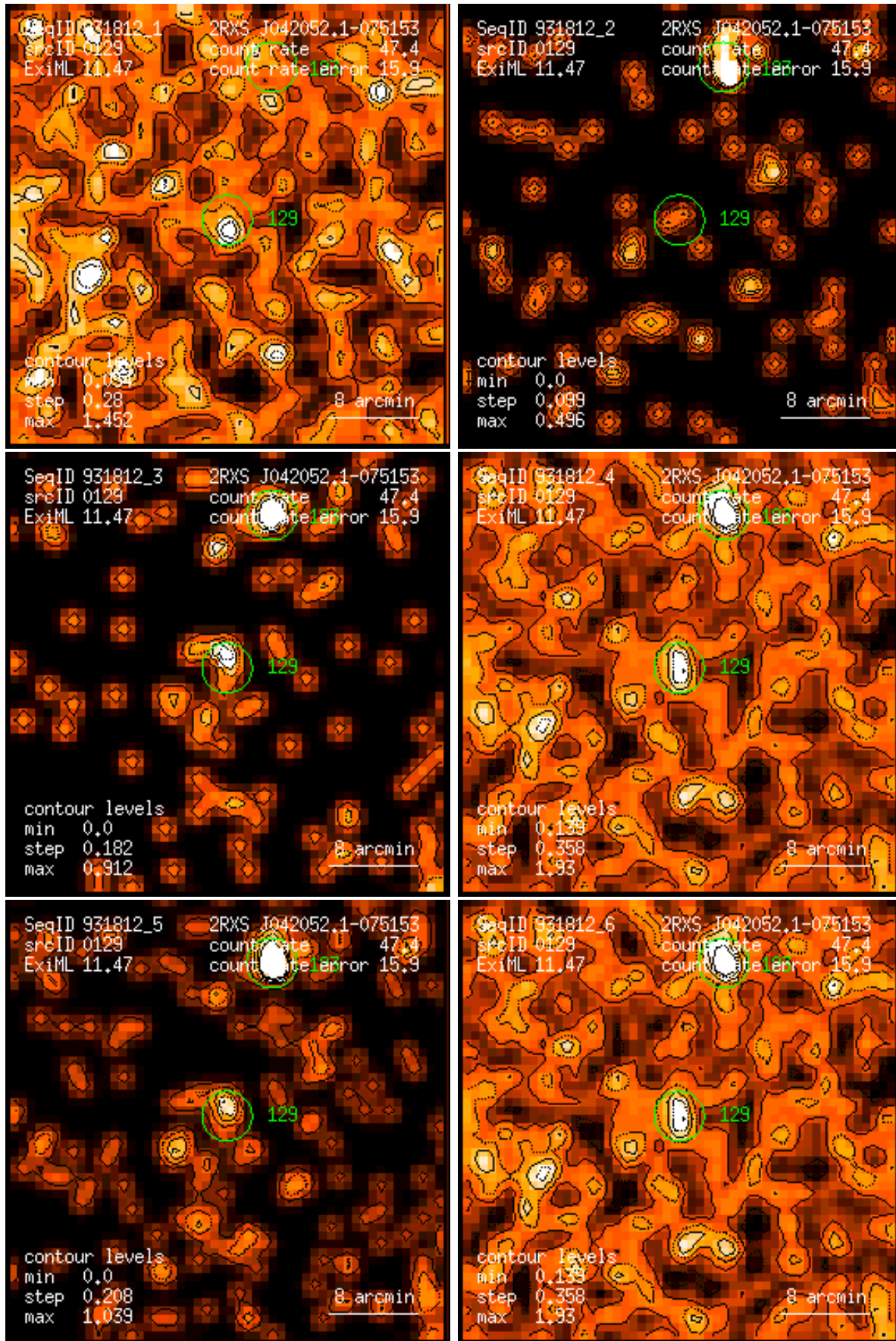
Figure 129: RASS 931812: detection 0129: band rate images, Gaussian filter: (1) PSPC channels 11 – 41, (2) 52 – 90, (3) 91 – 201, (4) 11 – 235, (5) 52 – 201, (6) 11 – 201. Broad band rates in counts/ks. Band rate contour levels in counts/ks/arcmin 2 .
