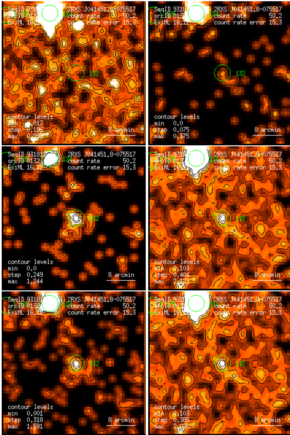
Figure 132: RASS 931812: detection 0132: band rate images, Gaussian filter: (1) PSPC channels 11 – 41, (2) 52 – 90, (3) 91 – 201, (4) 11 – 235, (5) 52 – 201, (6) 11 – 201. Broad band rates in counts/ks. Band rate contour levels in counts/ks/arcmin 2 .
