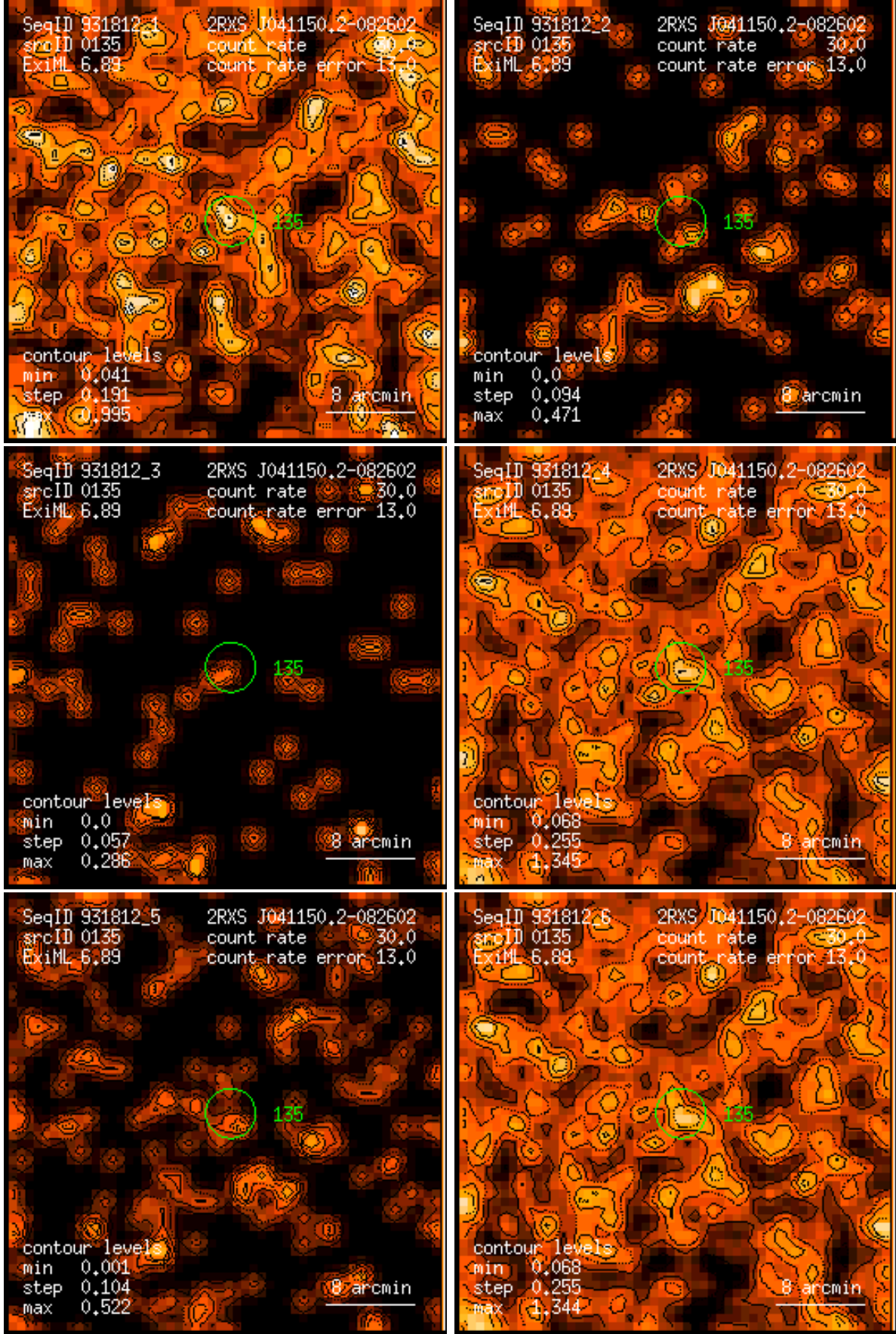
Figure 135: RASS 931812: detection 0135: band rate images, Gaussian filter: (1) PSPC channels 11 – 41, (2) 52 – 90, (3) 91 – 201, (4) 11 – 235, (5) 52 – 201, (6) 11 – 201. Broad band rates in counts/ks. Band rate contour levels in counts/ks/arcmin 2 .
