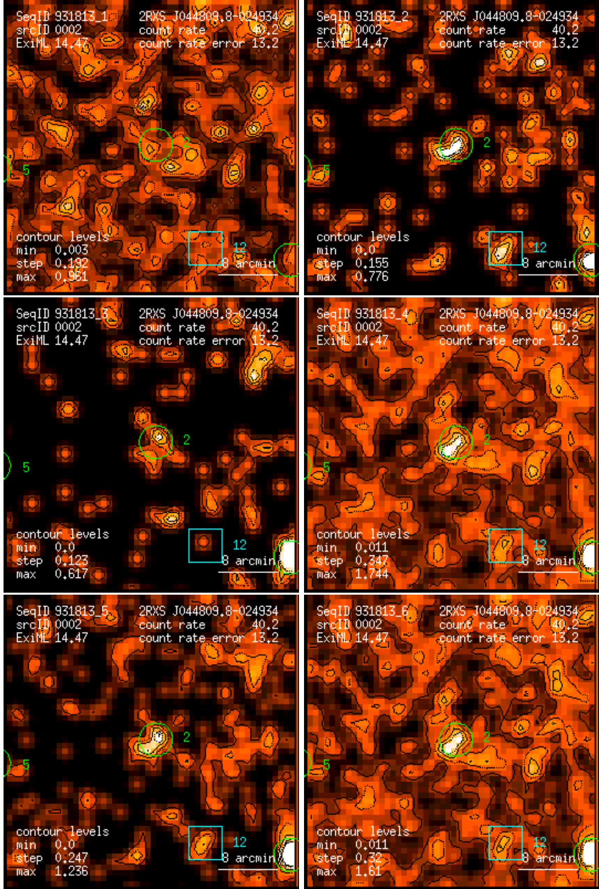
Figure 2: RASS 931813: detection 0002: band rate images, Gaussian filter: (1) PSPC channels 11 – 41, (2) 52 – 90, (3) 91 – 201, (4) 11 – 235, (5) 52 – 201, (6) 11 – 201. Broad band rates in counts/ks. Band rate contour levels in counts/ks/arcmin 2 .
