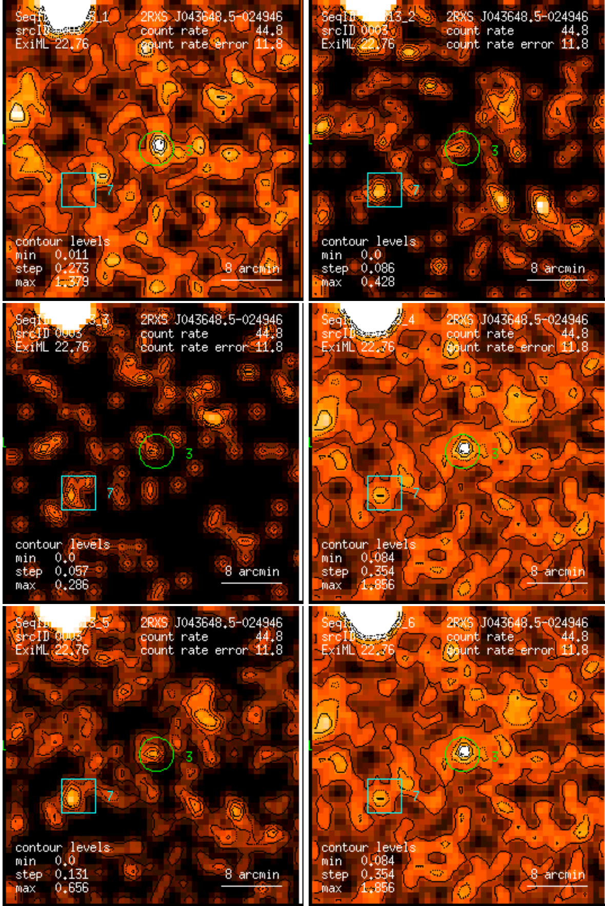
Figure 3: RASS 931813: detection 0003: band rate images, Gaussian filter: (1) PSPC channels 11 – 41, (2) 52 – 90, (3) 91 – 201, (4) 11 – 235, (5) 52 – 201, (6) 11 – 201. Broad band rates in counts/ks. Band rate contour levels in counts/ks/arcmin 2 .
