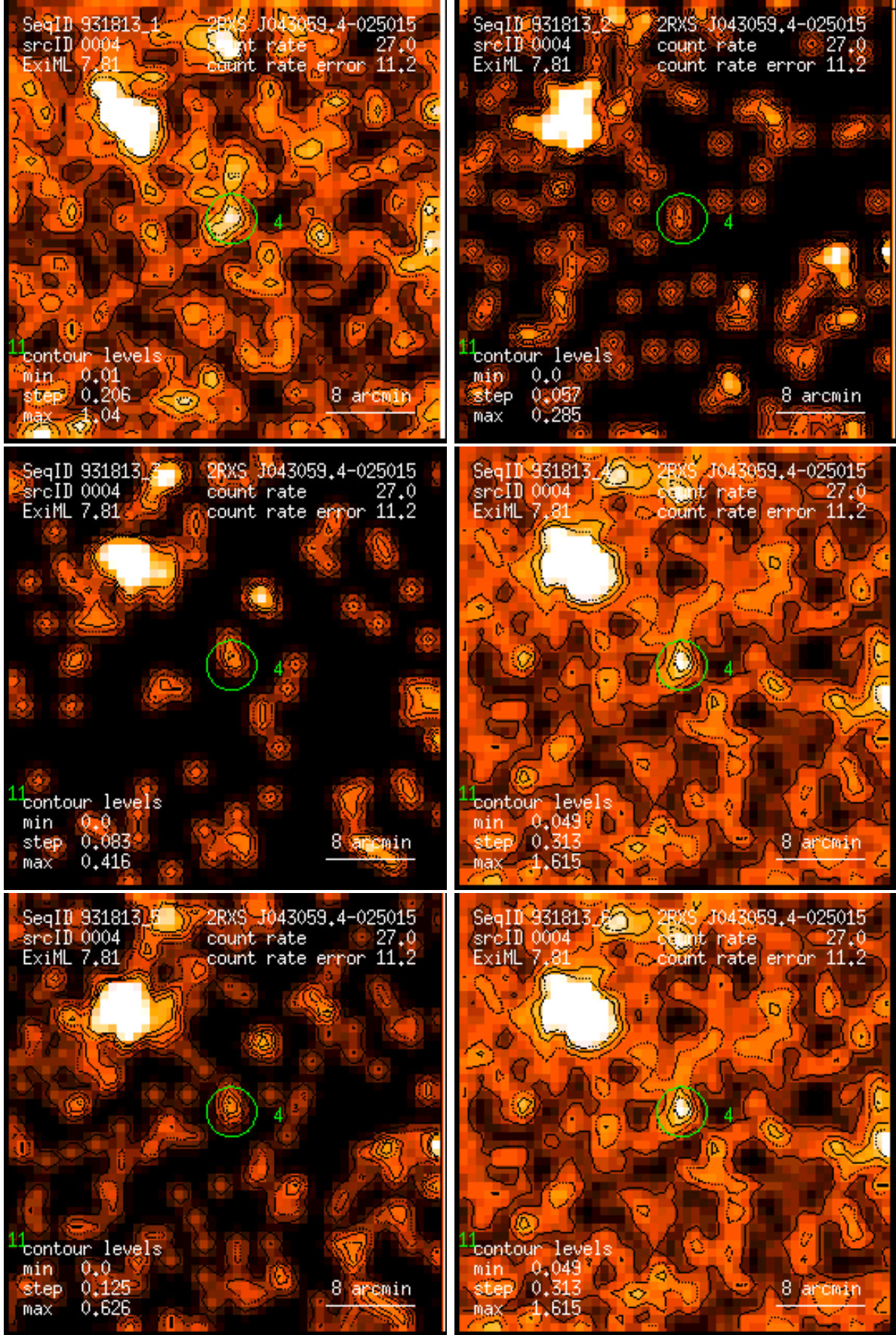
Figure 4: RASS 931813: detection 0004: band rate images, Gaussian filter: (1) PSPC channels 11 – 41, (2) 52 – 90, (3) 91 – 201, (4) 11 – 235, (5) 52 – 201, (6) 11 – 201. Broad band rates in counts/ks. Band rate contour levels in counts/ks/arcmin 2 .
