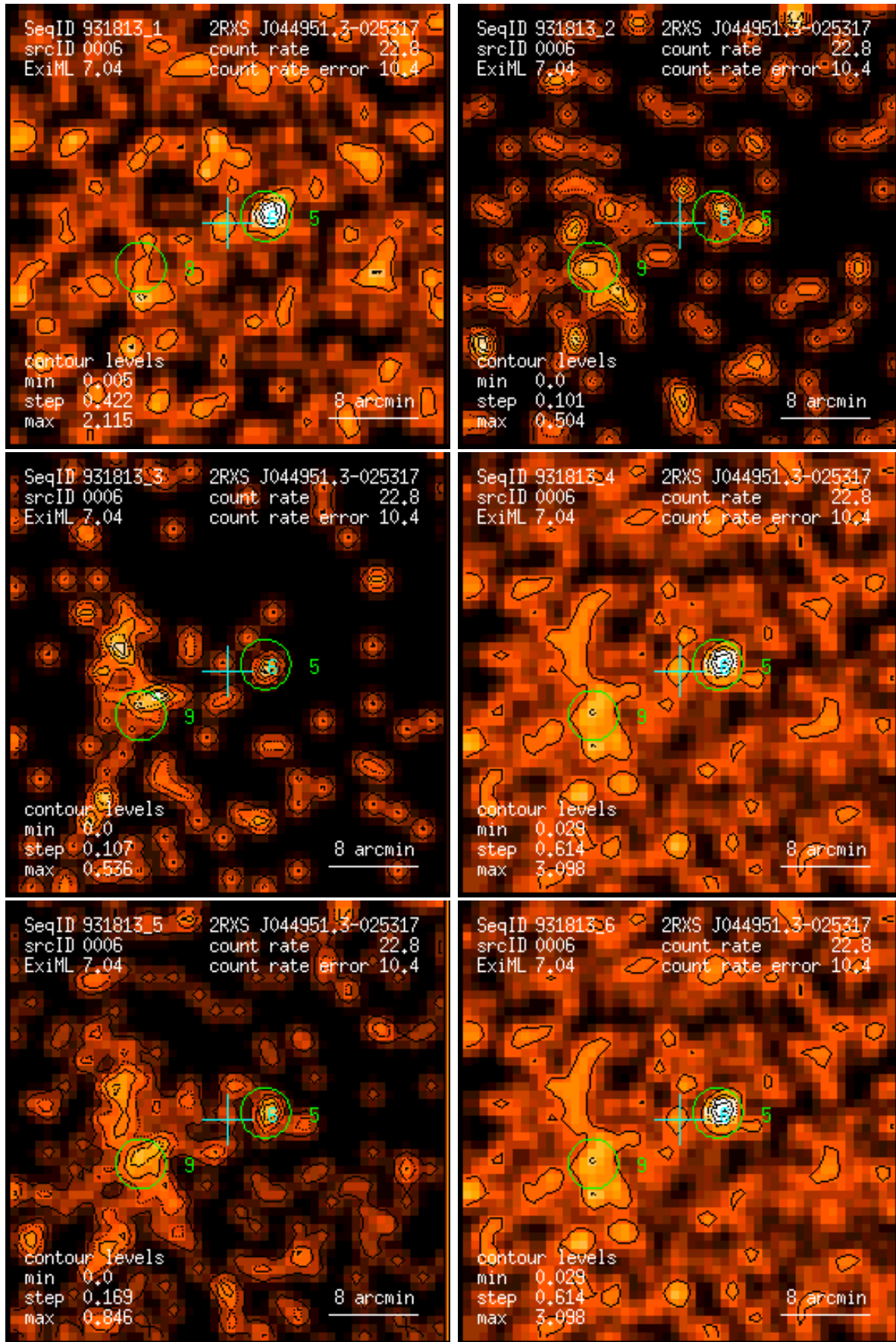
Figure 6: RASS 931813: detection 0006: band rate images, Gaussian filter: (1) PSPC channels 11 – 41, (2) 52 – 90, (3) 91 – 201, (4) 11 – 235, (5) 52 – 201, (6) 11 – 201. Broad band rates in counts/ks. Band rate contour levels in counts/ks/arcmin 2 .
