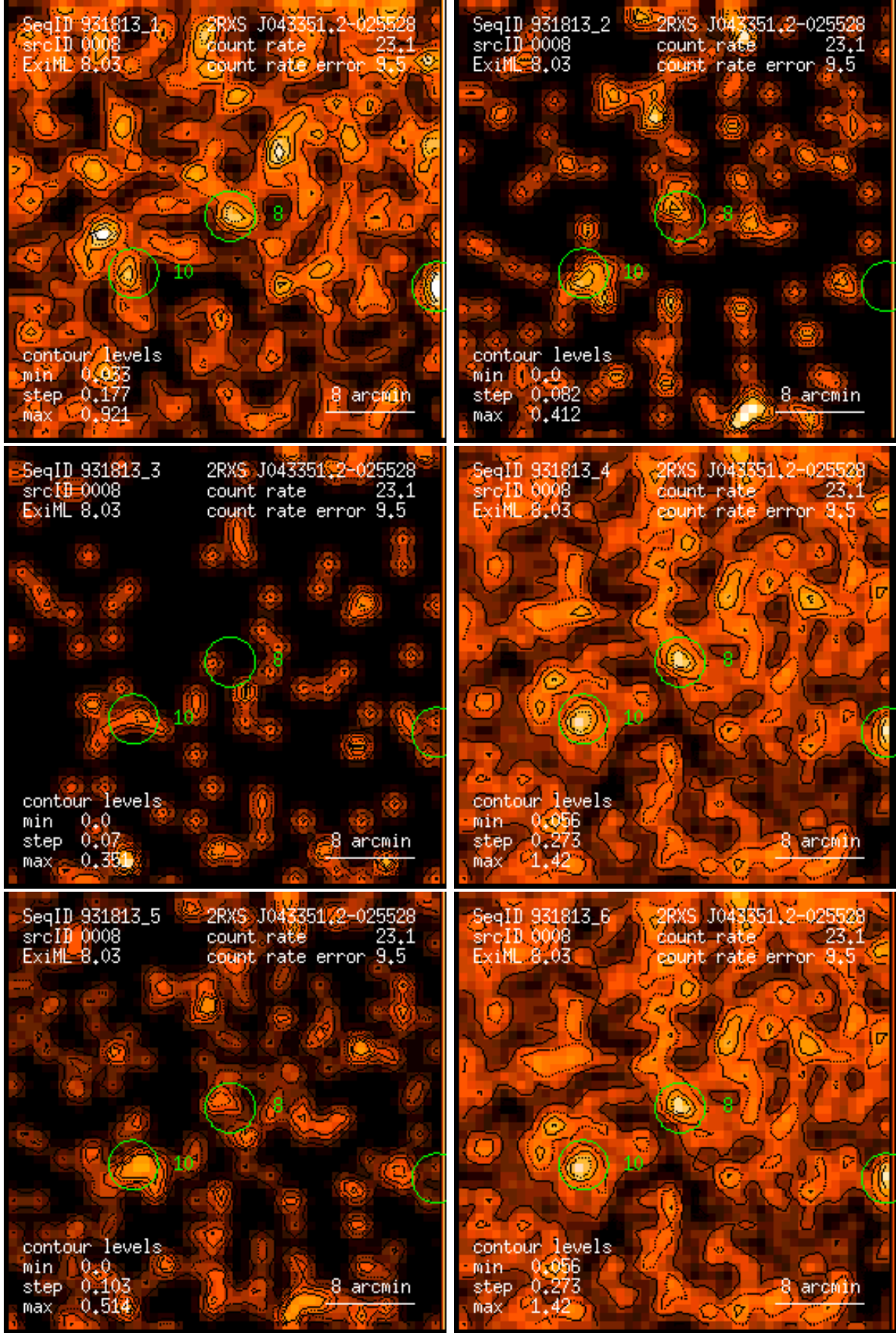
Figure 8: RASS 931813: detection 0008: band rate images, Gaussian filter: (1) PSPC channels 11 – 41, (2) 52 – 90, (3) 91 – 201, (4) 11 – 235, (5) 52 – 201, (6) 11 – 201. Broad band rates in counts/ks. Band rate contour levels in counts/ks/arcmin 2 .
