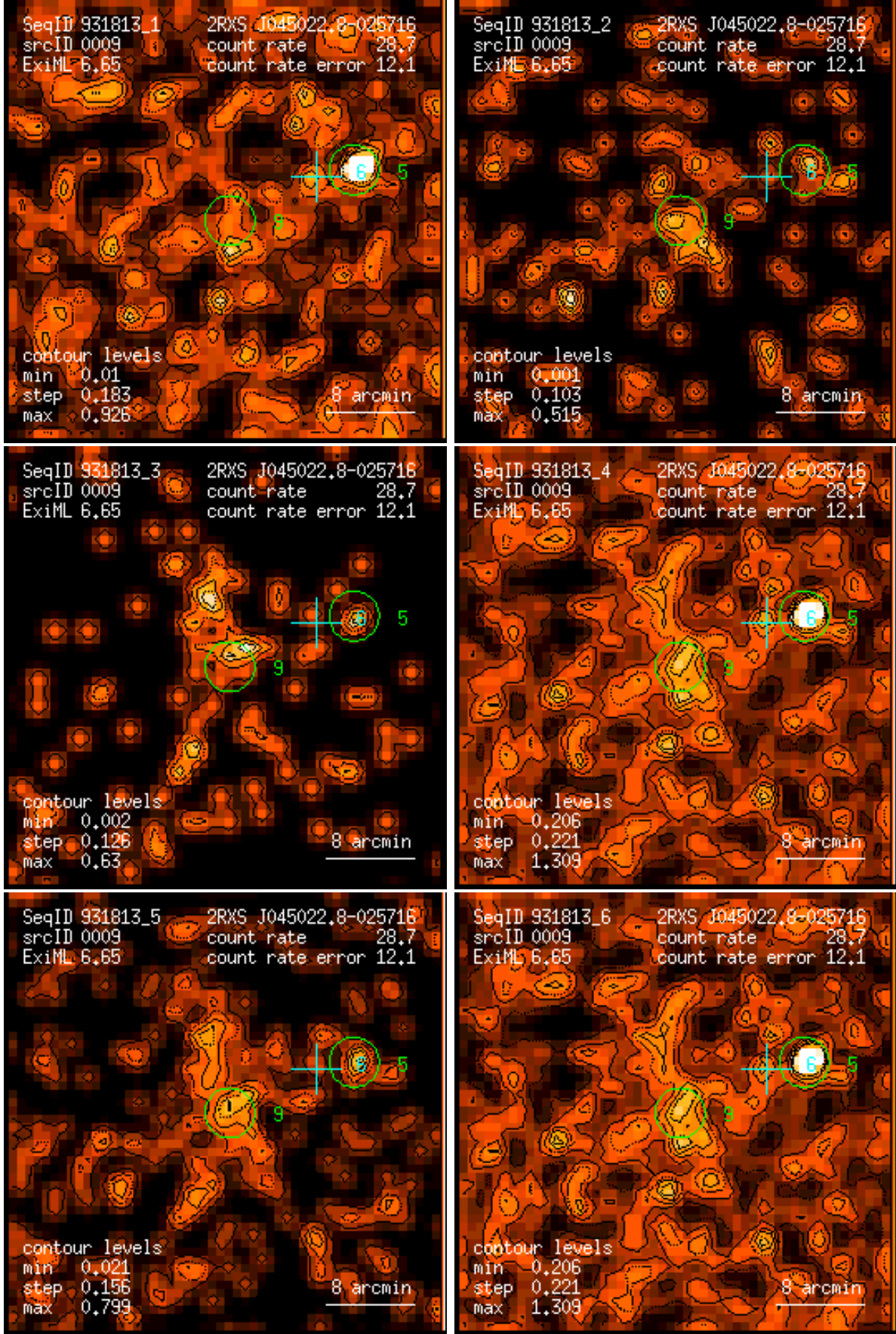
Figure 9: RASS 931813: detection 0009: band rate images, Gaussian filter: (1) PSPC channels 11 – 41, (2) 52 – 90, (3) 91 – 201, (4) 11 – 235, (5) 52 – 201, (6) 11 – 201. Broad band rates in counts/ks. Band rate contour levels in counts/ks/arcmin 2 .
