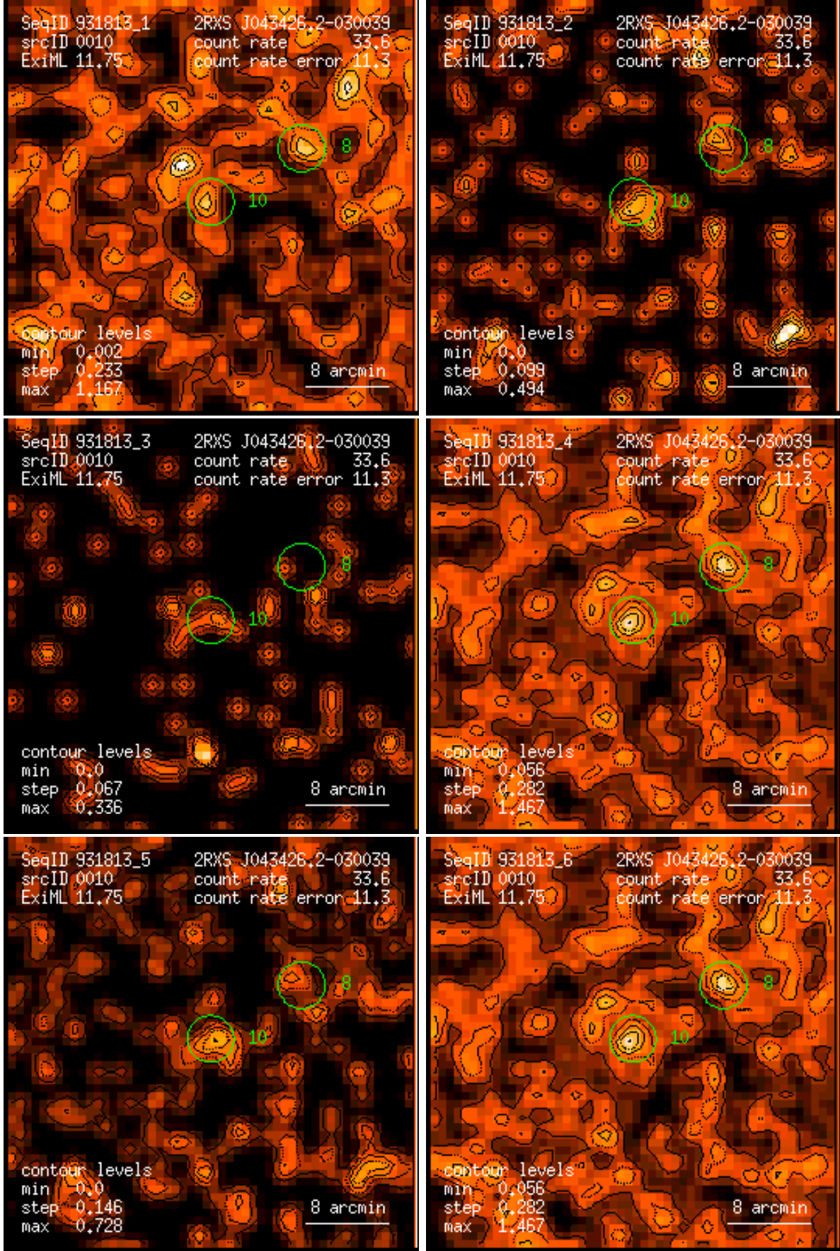
Figure 10: RASS 931813: detection 0010: band rate images, Gaussian filter: (1) PSPC channels 11 – 41, (2) 52 – 90, (3) 91 – 201, (4) 11 – 235, (5) 52 – 201, (6) 11 – 201. Broad band rates in counts/ks. Band rate contour levels in counts/ks/arcmin 2 .
