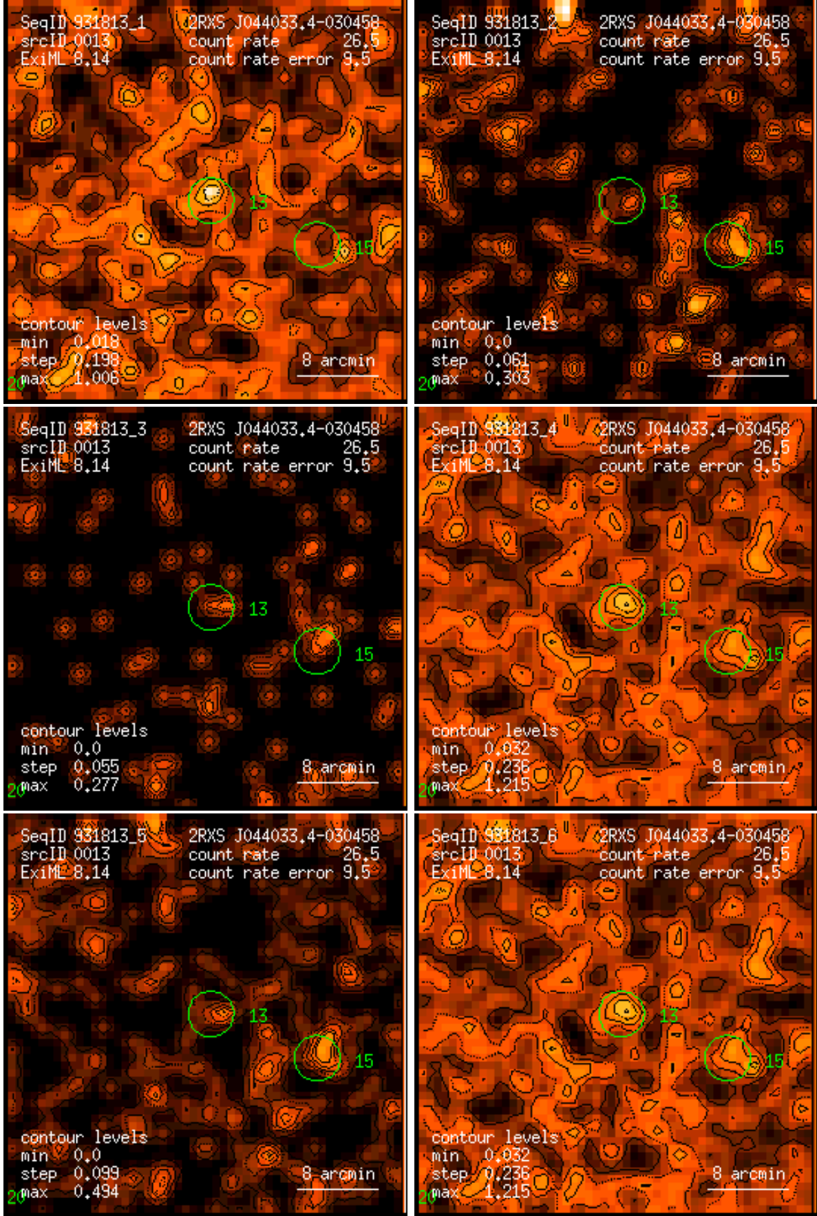
Figure 13: RASS 931813: detection 0013: band rate images, Gaussian filter: (1) PSPC channels 11 – 41, (2) 52 – 90, (3) 91 – 201, (4) 11 – 235, (5) 52 – 201, (6) 11 – 201. Broad band rates in counts/ks. Band rate contour levels in counts/ks/arcmin 2 .
