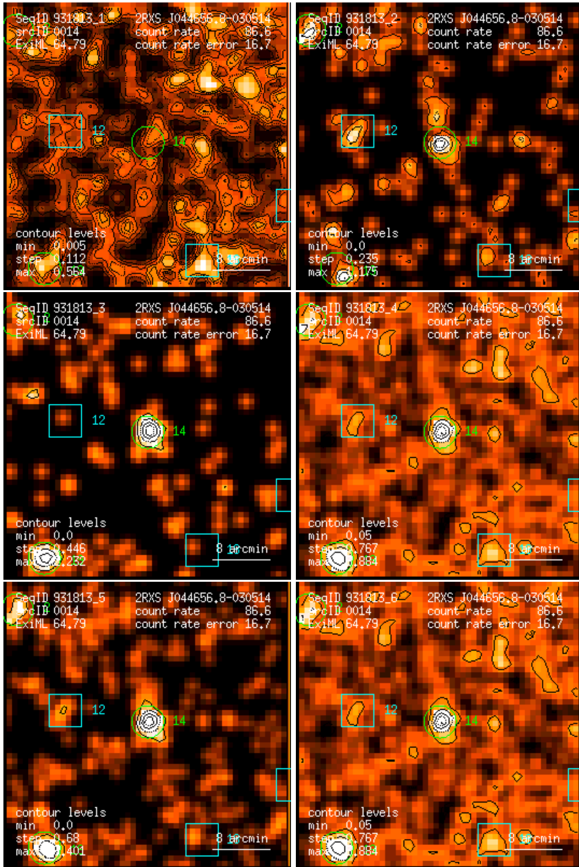
Figure 14: RASS 931813: detection 0014: band rate images, Gaussian filter: (1) PSPC channels 11 – 41, (2) 52 – 90, (3) 91 – 201, (4) 11 – 235, (5) 52 – 201, (6) 11 – 201. Broad band rates in counts/ks. Band rate contour levels in counts/ks/arcmin 2 .
