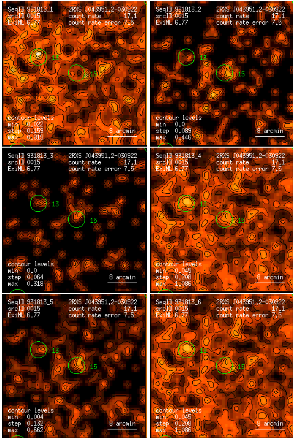
Figure 15: RASS 931813: detection 0015: band rate images, Gaussian filter: (1) PSPC channels 11 – 41, (2) 52 – 90, (3) 91 – 201, (4) 11 – 235, (5) 52 – 201, (6) 11 – 201. Broad band rates in counts/ks. Band rate contour levels in counts/ks/arcmin 2 .
