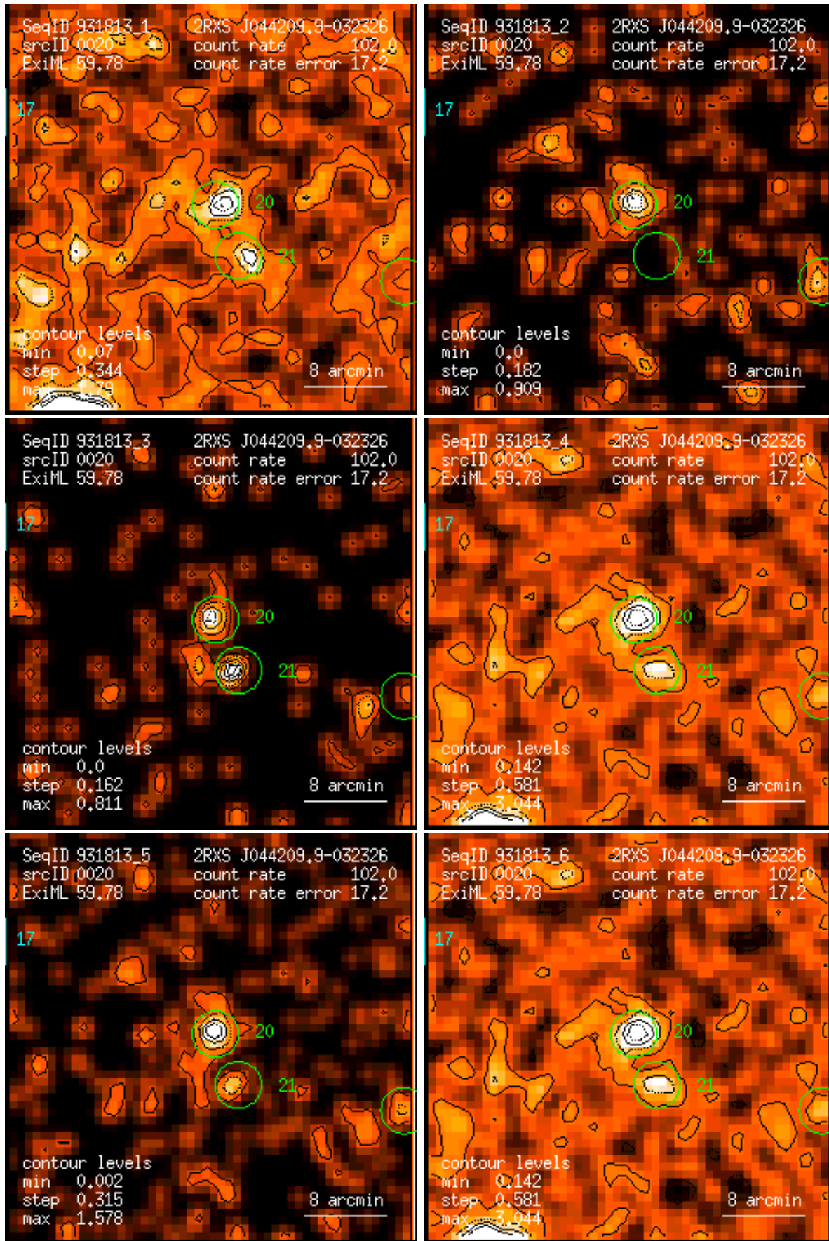
Figure 20: RASS 931813: detection 0020: band rate images, Gaussian filter: (1) PSPC channels 11 – 41, (2) 52 – 90, (3) 91 – 201, (4) 11 – 235, (5) 52 – 201, (6) 11 – 201. Broad band rates in counts/ks. Band rate contour levels in counts/ks/arcmin 2 .
