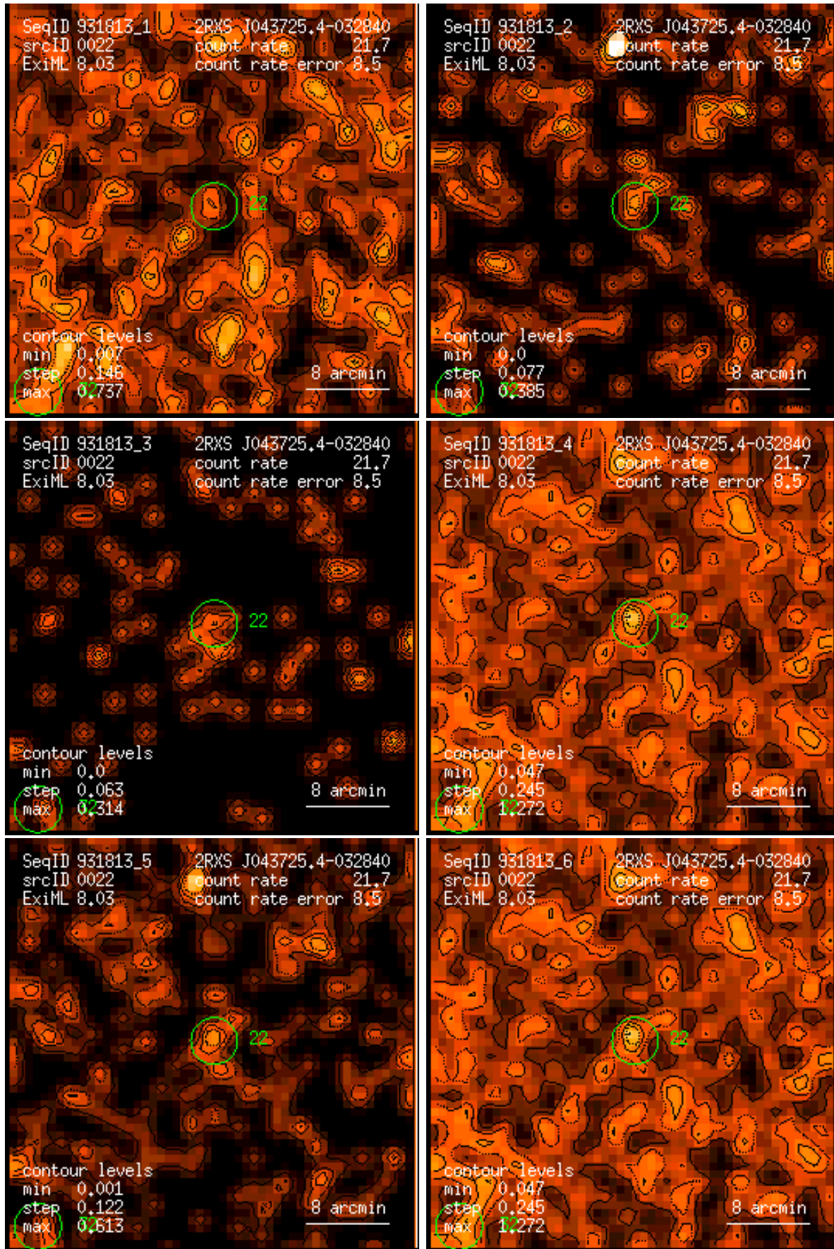
Figure 22: RASS 931813: detection 0022: band rate images, Gaussian filter: (1) PSPC channels 11 – 41, (2) 52 – 90, (3) 91 – 201, (4) 11 – 235, (5) 52 – 201, (6) 11 – 201. Broad band rates in counts/ks. Band rate contour levels in counts/ks/arcmin 2 .
