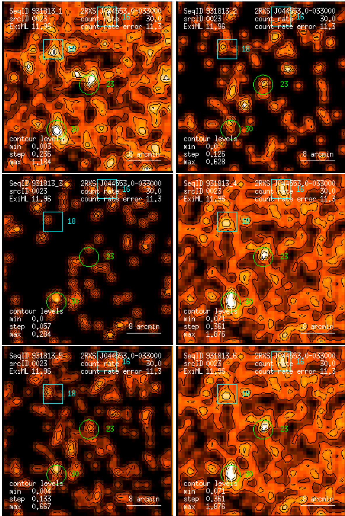
Figure 23: RASS 931813: detection 0023: band rate images, Gaussian filter: (1) PSPC channels 11 – 41, (2) 52 – 90, (3) 91 – 201, (4) 11 – 235, (5) 52 – 201, (6) 11 – 201. Broad band rates in counts/ks. Band rate contour levels in counts/ks/arcmin 2 .
