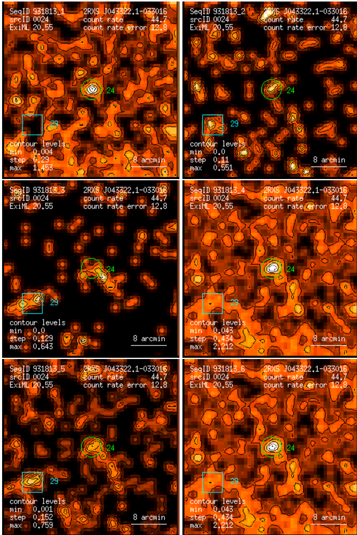
Figure 24: RASS 931813: detection 0024: band rate images, Gaussian filter: (1) PSPC channels 11 – 41, (2) 52 – 90, (3) 91 – 201, (4) 11 – 235, (5) 52 – 201, (6) 11 – 201. Broad band rates in counts/ks. Band rate contour levels in counts/ks/arcmin 2 .
