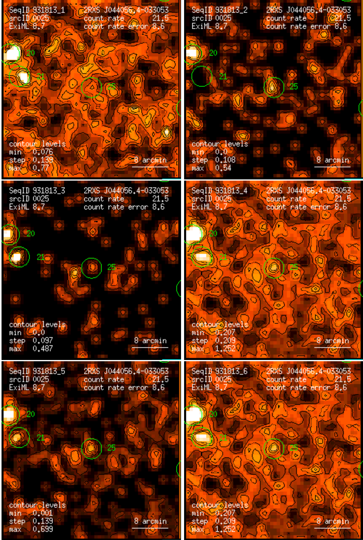
Figure 25: RASS 931813: detection 0025: band rate images, Gaussian filter: (1) PSPC channels 11 – 41, (2) 52 – 90, (3) 91 – 201, (4) 11 – 235, (5) 52 – 201, (6) 11 – 201. Broad band rates in counts/ks. Band rate contour levels in counts/ks/arcmin 2 .
