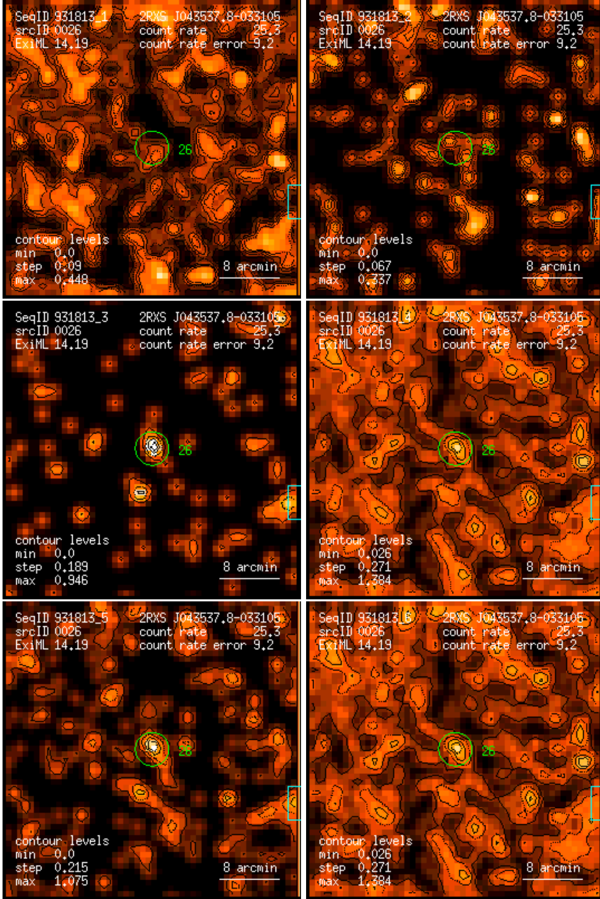
Figure 26: RASS 931813: detection 0026: band rate images, Gaussian filter: (1) PSPC channels 11 – 41, (2) 52 – 90, (3) 91 – 201, (4) 11 – 235, (5) 52 – 201, (6) 11 – 201. Broad band rates in counts/ks. Band rate contour levels in counts/ks/arcmin 2 .
