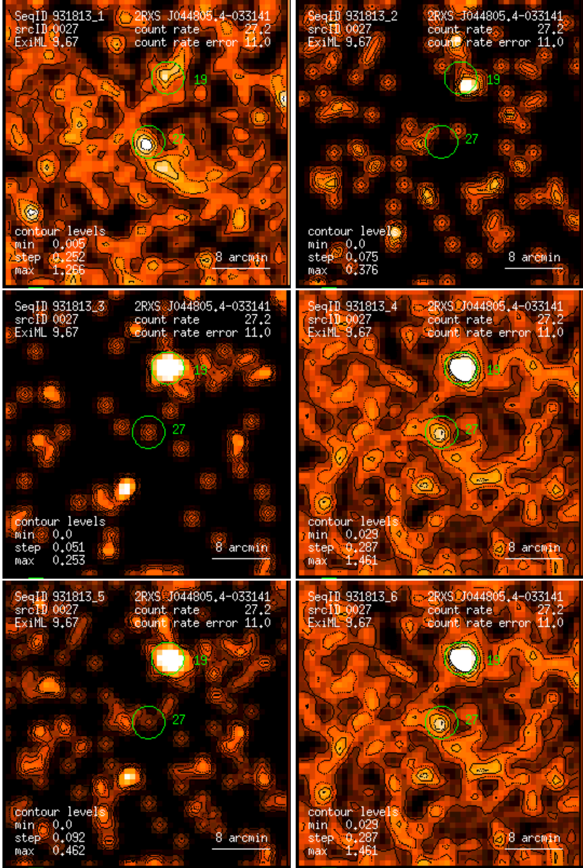
Figure 27: RASS 931813: detection 0027: band rate images, Gaussian filter: (1) PSPC channels 11 – 41, (2) 52 – 90, (3) 91 – 201, (4) 11 – 235, (5) 52 – 201, (6) 11 – 201. Broad band rates in counts/ks. Band rate contour levels in counts/ks/arcmin 2 .
