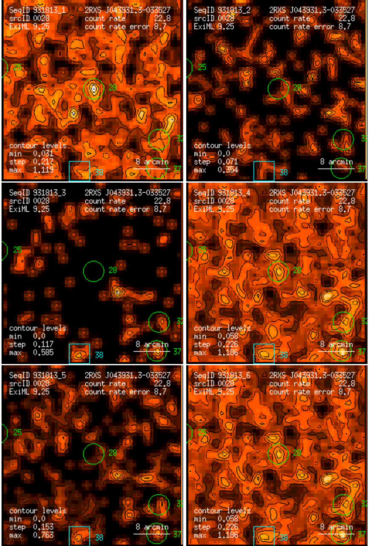
Figure 28: RASS 931813: detection 0028: band rate images, Gaussian filter: (1) PSPC channels 11 – 41, (2) 52 – 90, (3) 91 – 201, (4) 11 – 235, (5) 52 – 201, (6) 11 – 201. Broad band rates in counts/ks. Band rate contour levels in counts/ks/arcmin 2 .
