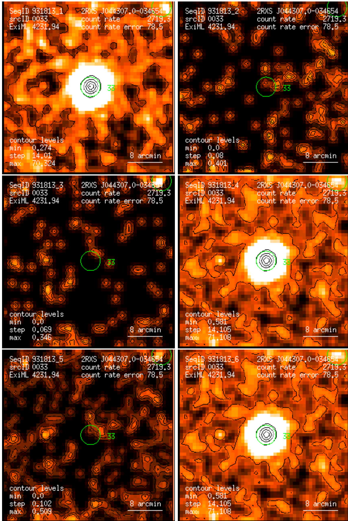
Figure 33: RASS 931813: detection 0033: band rate images, Gaussian filter: (1) PSPC channels 11 – 41, (2) 52 – 90, (3) 91 – 201, (4) 11 – 235, (5) 52 – 201, (6) 11 – 201. Broad band rates in counts/ks. Band rate contour levels in counts/ks/arcmin 2 .
