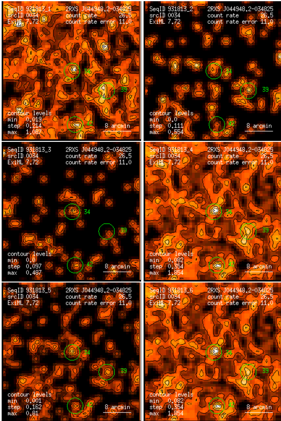
Figure 34: RASS 931813: detection 0034: band rate images, Gaussian filter: (1) PSPC channels 11 – 41, (2) 52 – 90, (3) 91 – 201, (4) 11 – 235, (5) 52 – 201, (6) 11 – 201. Broad band rates in counts/ks. Band rate contour levels in counts/ks/arcmin 2 .
