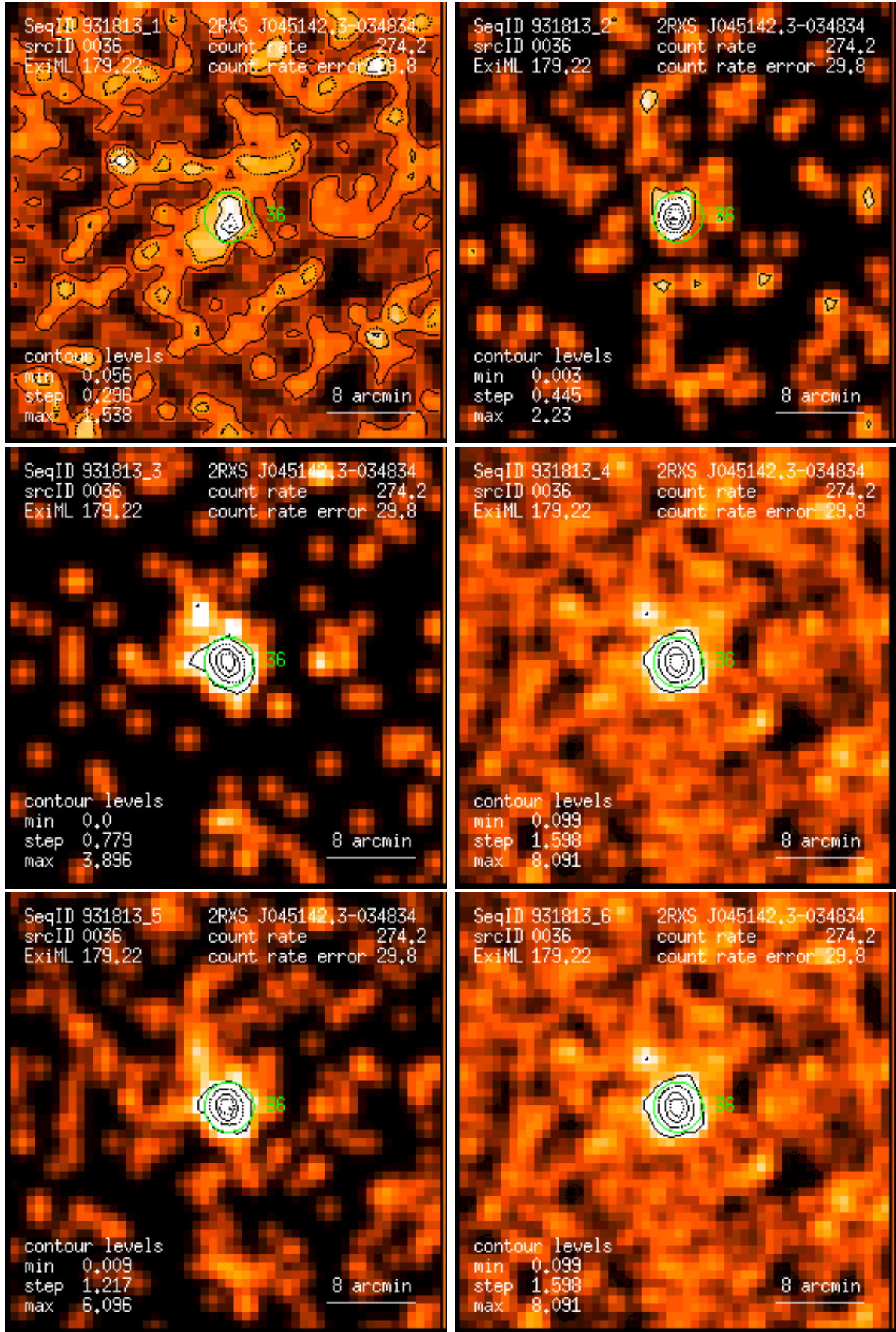
Figure 36: RASS 931813: detection 0036: band rate images, Gaussian filter: (1) PSPC channels 11 – 41, (2) 52 – 90, (3) 91 – 201, (4) 11 – 235, (5) 52 – 201, (6) 11 – 201. Broad band rates in counts/ks. Band rate contour levels in counts/ks/arcmin 2 .
