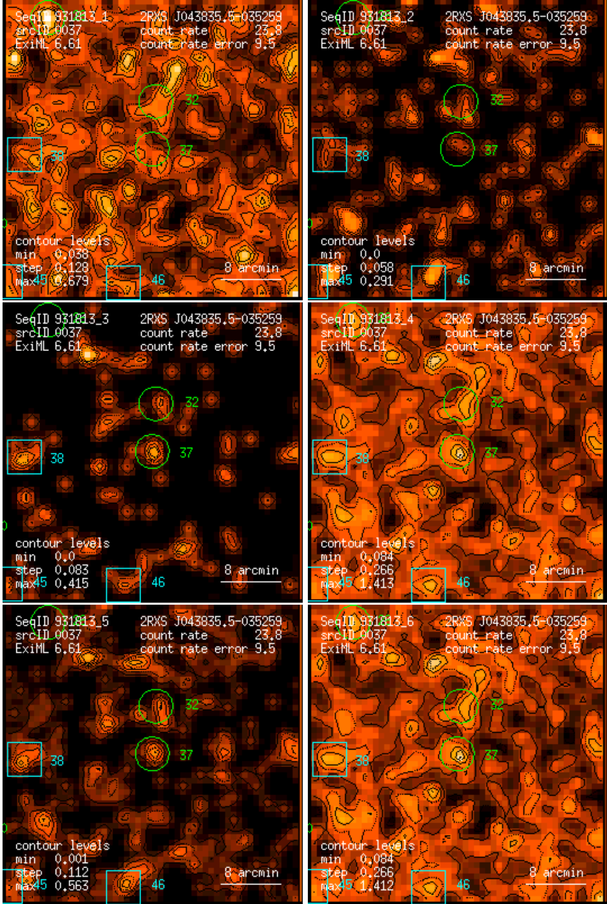
Figure 37: RASS 931813: detection 0037: band rate images, Gaussian filter: (1) PSPC channels 11 – 41, (2) 52 – 90, (3) 91 – 201, (4) 11 – 235, (5) 52 – 201, (6) 11 – 201. Broad band rates in counts/ks. Band rate contour levels in counts/ks/arcmin 2 .
