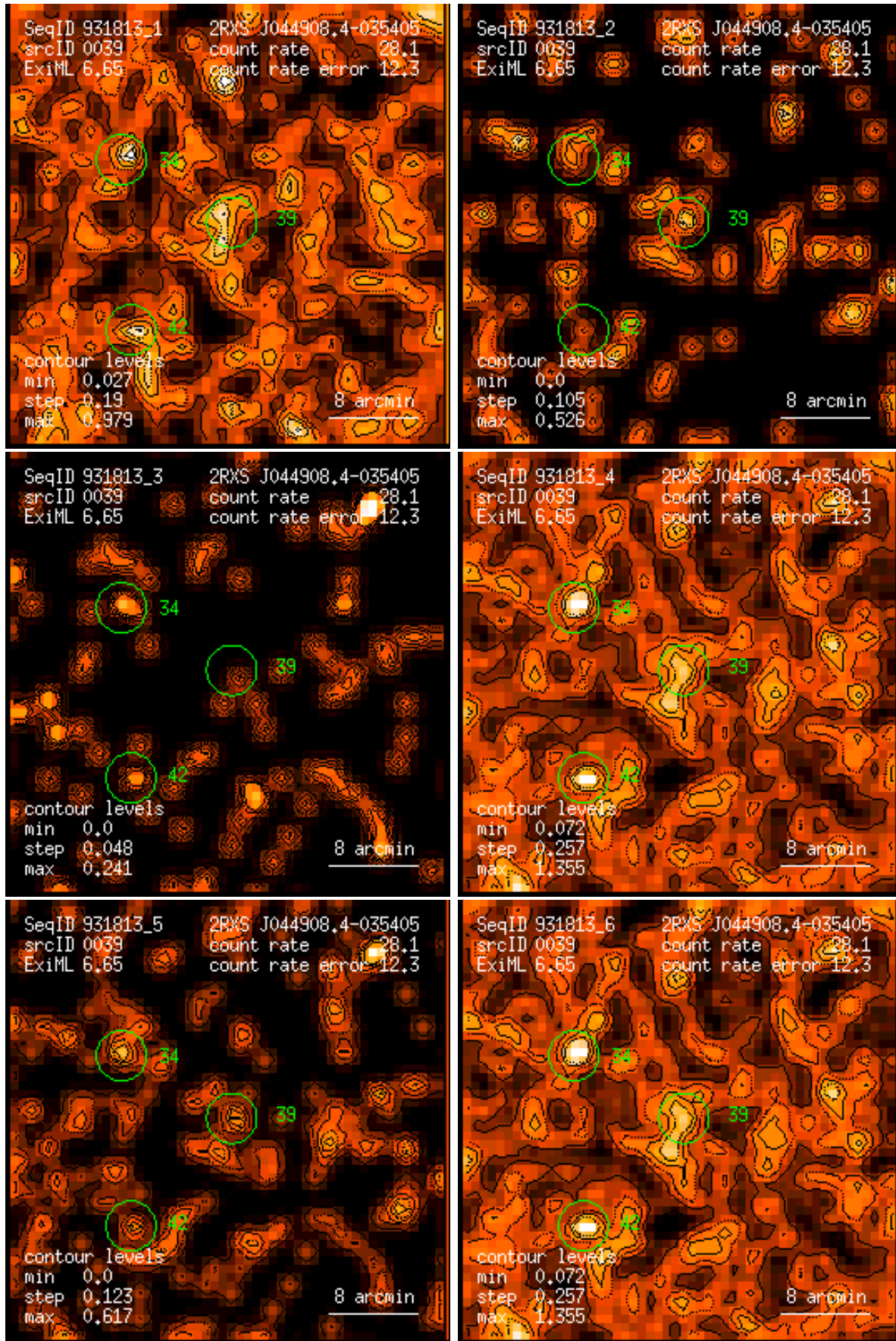
Figure 39: RASS 931813: detection 0039: band rate images, Gaussian filter: (1) PSPC channels 11 – 41, (2) 52 – 90, (3) 91 – 201, (4) 11 – 235, (5) 52 – 201, (6) 11 – 201. Broad band rates in counts/ks. Band rate contour levels in counts/ks/arcmin 2 .
