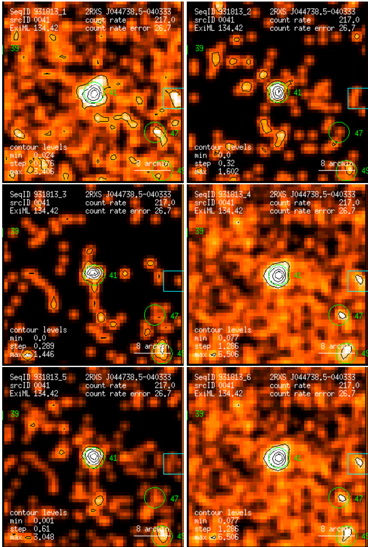
Figure 41: RASS 931813: detection 0041: band rate images, Gaussian filter: (1) PSPC channels 11 – 41, (2) 52 – 90, (3) 91 – 201, (4) 11 – 235, (5) 52 – 201, (6) 11 – 201. Broad band rates in counts/ks. Band rate contour levels in counts/ks/arcmin 2 .
