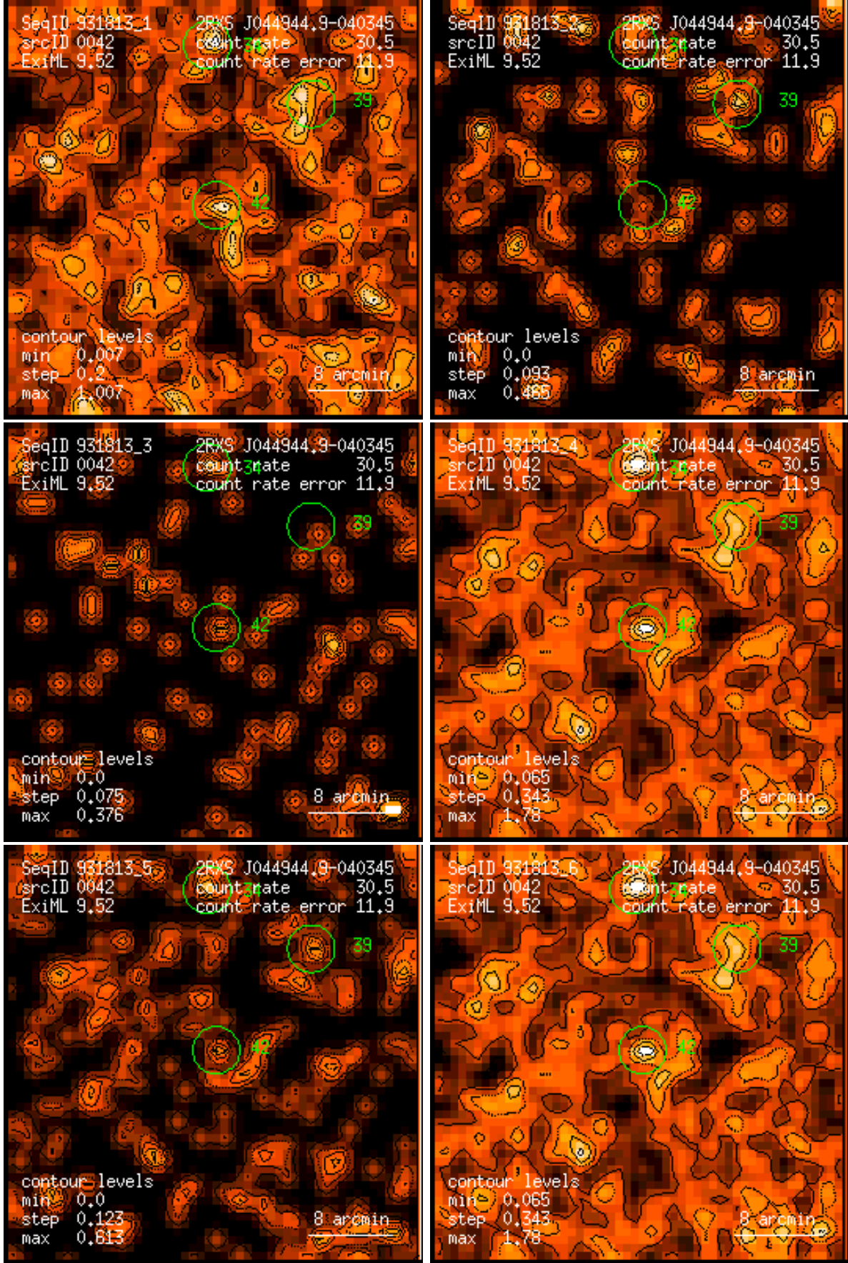
Figure 42: RASS 931813: detection 0042: band rate images, Gaussian filter: (1) PSPC channels 11 – 41, (2) 52 – 90, (3) 91 – 201, (4) 11 – 235, (5) 52 – 201, (6) 11 – 201. Broad band rates in counts/ks. Band rate contour levels in counts/ks/arcmin 2 .
