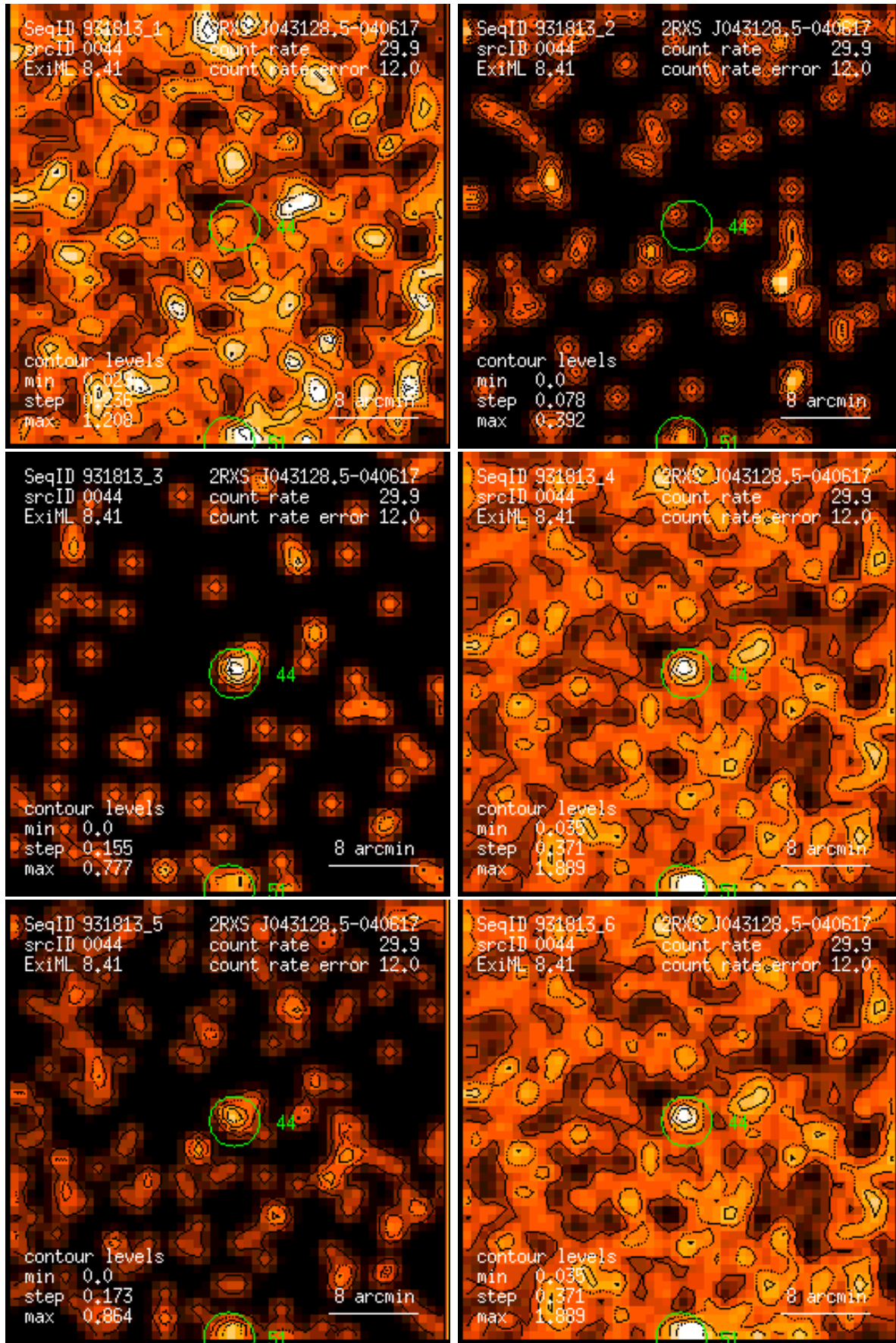
Figure 44: RASS 931813: detection 0044: band rate images, Gaussian filter: (1) PSPC channels 11 – 41, (2) 52 – 90, (3) 91 – 201, (4) 11 – 235, (5) 52 – 201, (6) 11 – 201. Broad band rates in counts/ks. Band rate contour levels in counts/ks/arcmin 2 .
