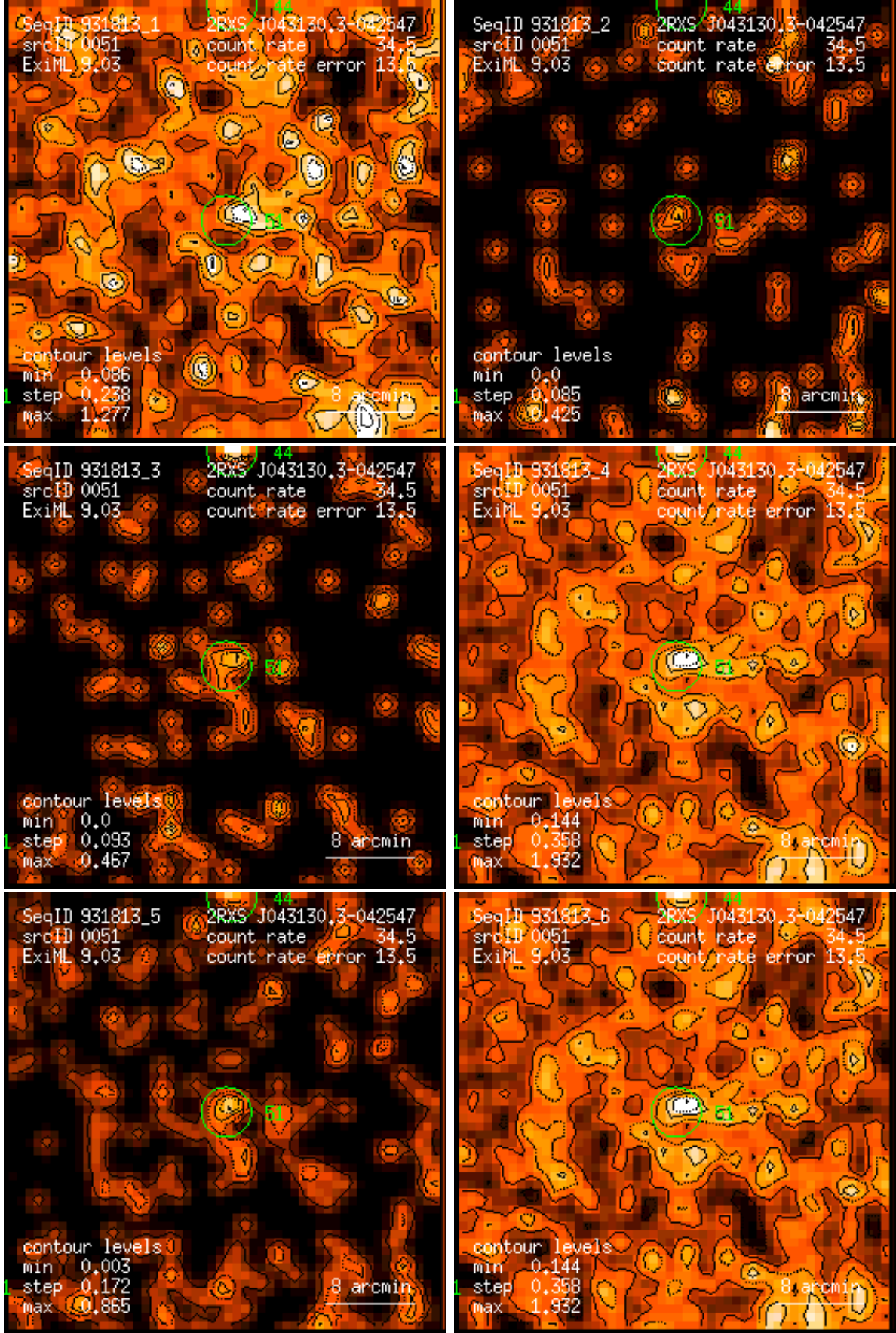
Figure 51: RASS 931813: detection 0051: band rate images, Gaussian filter: (1) PSPC channels 11 – 41, (2) 52 – 90, (3) 91 – 201, (4) 11 – 235, (5) 52 – 201, (6) 11 – 201. Broad band rates in counts/ks. Band rate contour levels in counts/ks/arcmin 2 .
