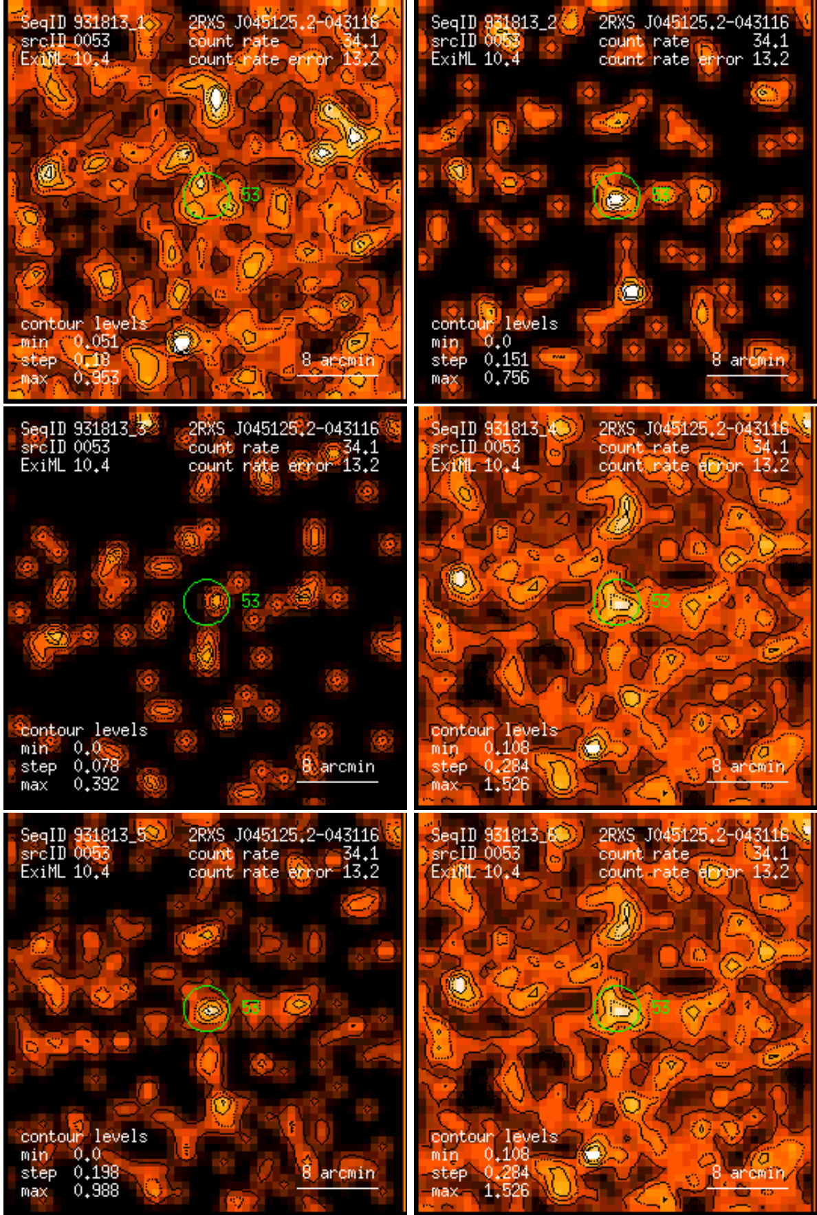
Figure 53: RASS 931813: detection 0053: band rate images, Gaussian filter: (1) PSPC channels 11 – 41, (2) 52 – 90, (3) 91 – 201, (4) 11 – 235, (5) 52 – 201, (6) 11 – 201. Broad band rates in counts/ks. Band rate contour levels in counts/ks/arcmin 2 .
