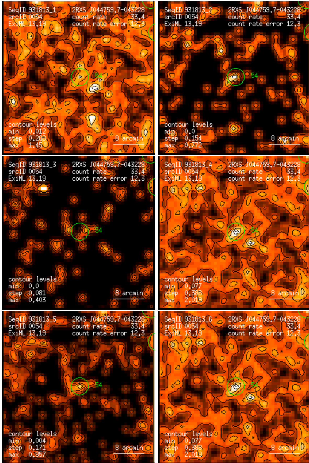
Figure 54: RASS 931813: detection 0054: band rate images, Gaussian filter: (1) PSPC channels 11 – 41, (2) 52 – 90, (3) 91 – 201, (4) 11 – 235, (5) 52 – 201, (6) 11 – 201. Broad band rates in counts/ks. Band rate contour levels in counts/ks/arcmin 2 .
