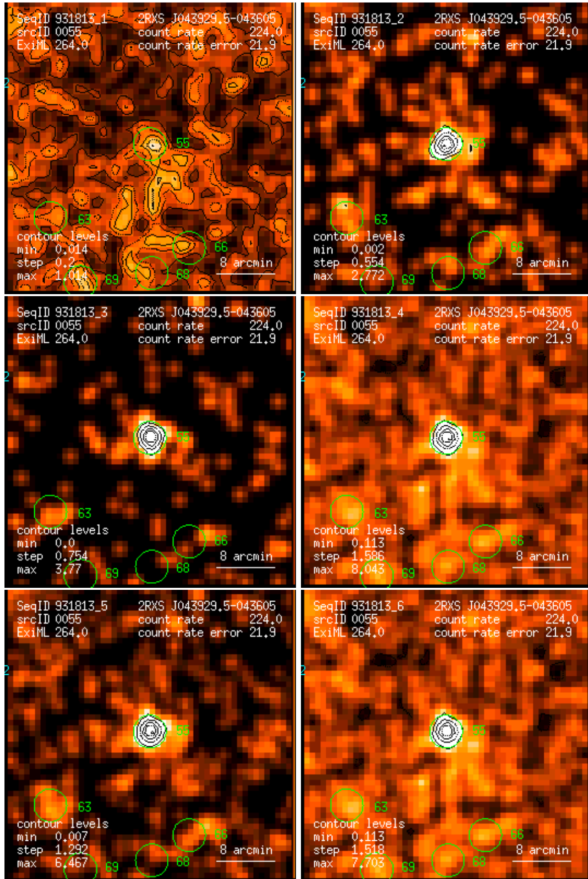
Figure 55: RASS 931813: detection 0055: band rate images, Gaussian filter: (1) PSPC channels 11 – 41, (2) 52 – 90, (3) 91 – 201, (4) 11 – 235, (5) 52 – 201, (6) 11 – 201. Broad band rates in counts/ks. Band rate contour levels in counts/ks/arcmin 2 .
