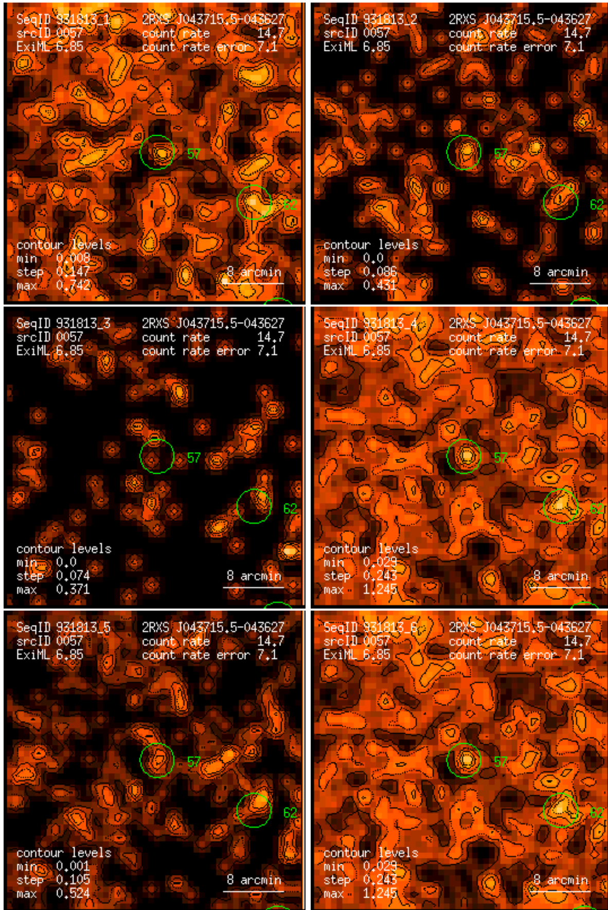
Figure 57: RASS 931813: detection 0057: band rate images, Gaussian filter: (1) PSPC channels 11 – 41, (2) 52 – 90, (3) 91 – 201, (4) 11 – 235, (5) 52 – 201, (6) 11 – 201. Broad band rates in counts/ks. Band rate contour levels in counts/ks/arcmin 2 .
