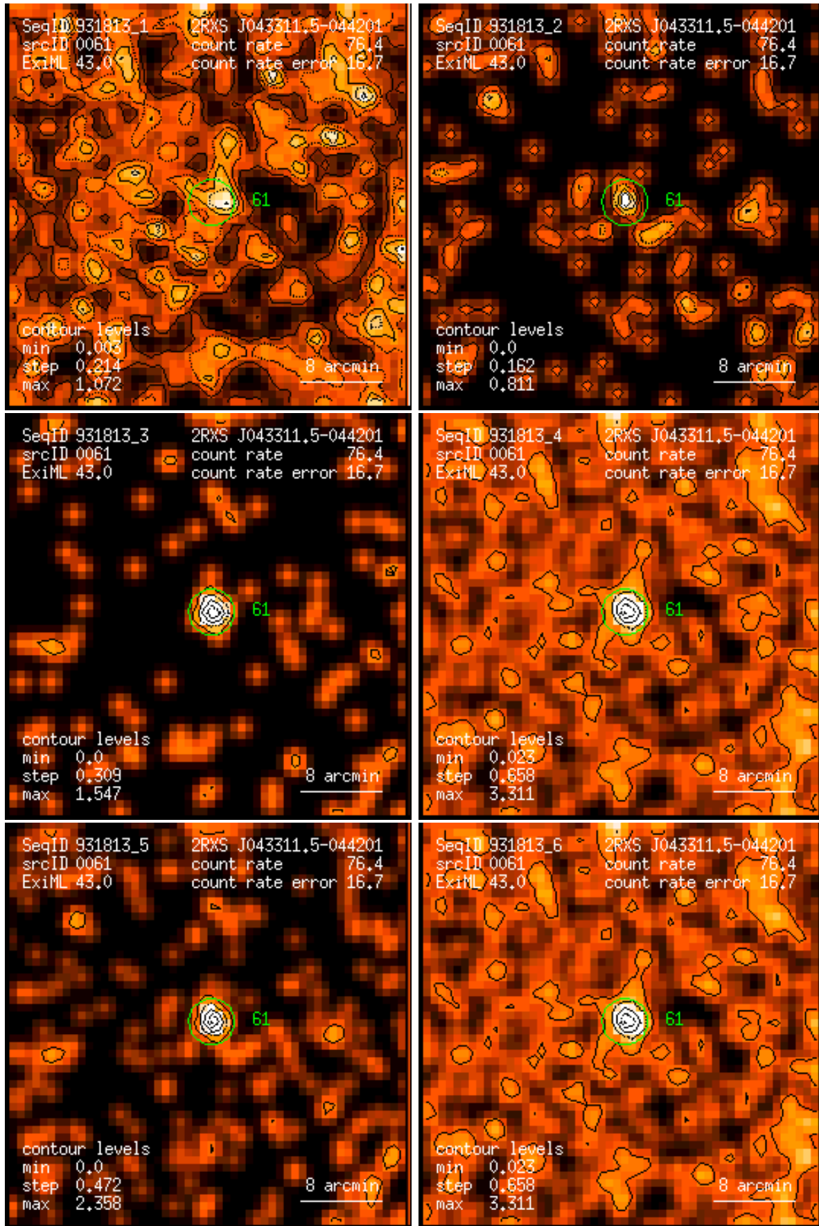
Figure 61: RASS 931813: detection 0061: band rate images, Gaussian filter: (1) PSPC channels 11 – 41, (2) 52 – 90, (3) 91 – 201, (4) 11 – 235, (5) 52 – 201, (6) 11 – 201. Broad band rates in counts/ks. Band rate contour levels in counts/ks/arcmin 2 .
