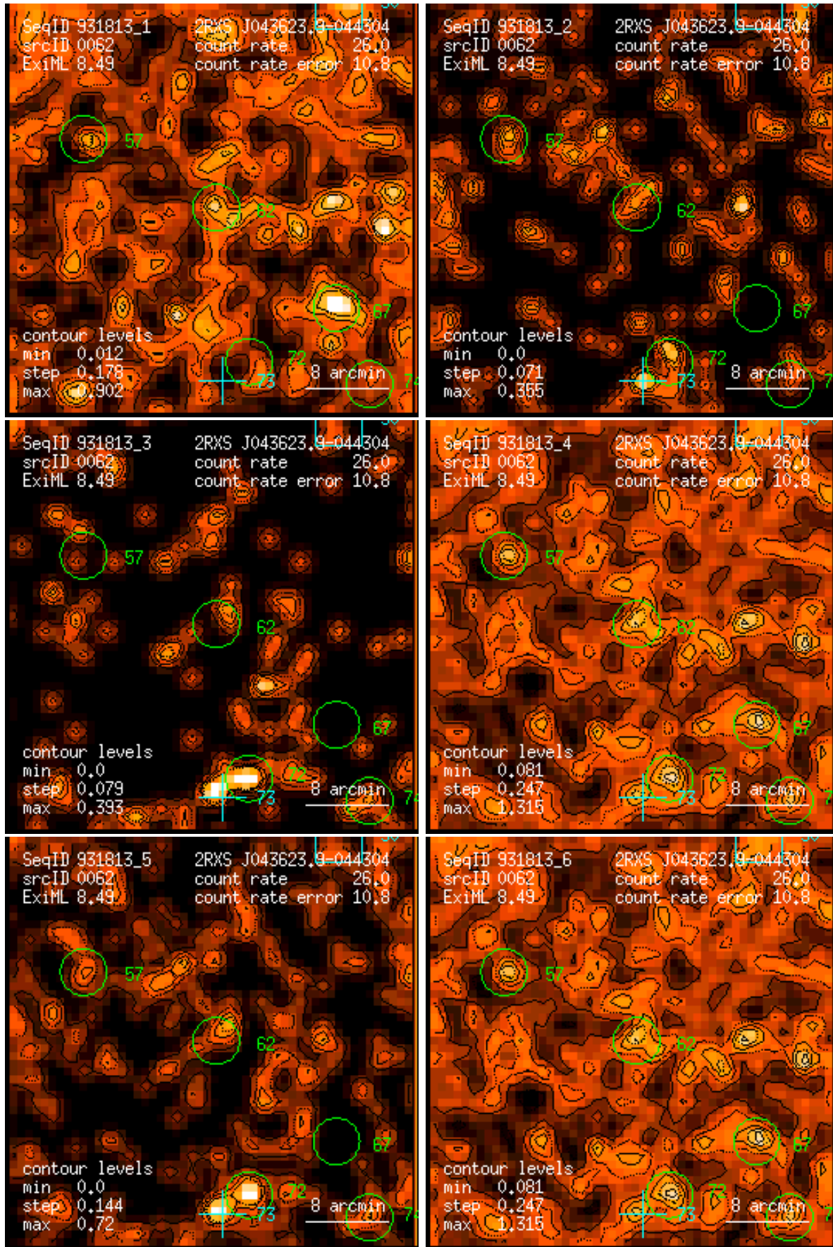
Figure 62: RASS 931813: detection 0062: band rate images, Gaussian filter: (1) PSPC channels 11 – 41, (2) 52 – 90, (3) 91 – 201, (4) 11 – 235, (5) 52 – 201, (6) 11 – 201. Broad band rates in counts/ks. Band rate contour levels in counts/ks/arcmin 2 .
